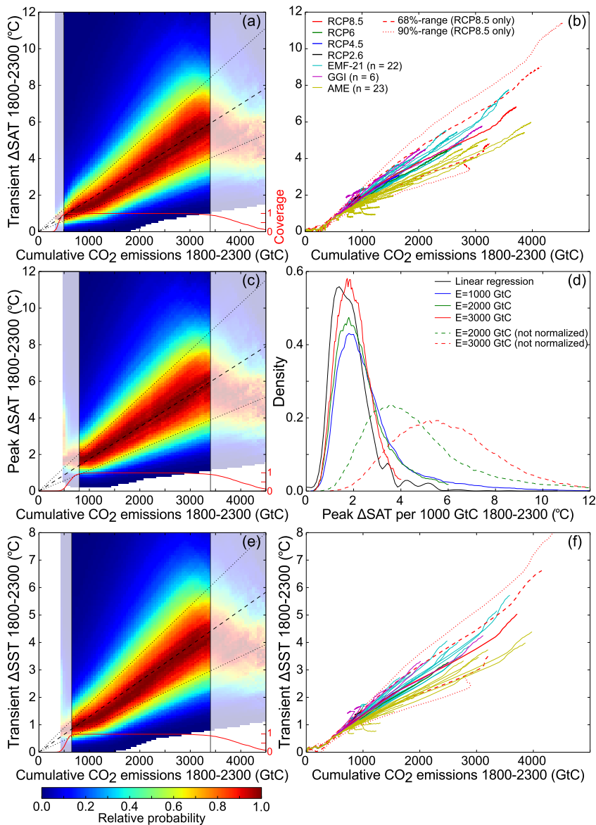
Figure 3. Transient and peak warming as function of cumulative emissions: (a) relative probability of transient surface air temperature change ( \Delta SAT) for given cumulative CO 2 emissions (fossil fuel and deforestation), derived from annual values from ensemble model simulations for 55 greenhouse-gas emission scenarios. Black dashed lines show the median and 68 %-range of the linear regression slope. The red line indicates the coverage of the emission range by the model ensemble. High and low emission ranges with a coverage of less than 90 % are shaded and considered not robust. (b) Transient \Delta SAT response (ensemble median) for the 55 different scenarios. The dashed/dotted lines show the 68/90 %-range of the ensemble for the RCP8.5 scenario, to indicate the model-spread. Please note that our extensions of the RCP scenarios beyond 2100 are not identical to the Extended Concentration Pathways (ECP, see Methods). (c) Same as (a) but for the peak warming for given total cumulative emissions. (d) PDFs of the peak warming for 1000 (blue), 2000 (green), and 3000 Gt C (red) cumulative emissions, and for the linear regression (black). The dashed lines indicate the unscaled PDFs and solid lines the normalized response per 1000 Gt C. (e, f) Same as (a, b) but for transient sea surface temperature change ( \Delta SST).
