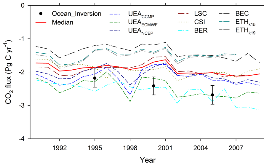
Fig. 6. Summary of annual global-integrated sea-air CO 2 fluxes from the ocean general circulation models, OGCMs (dashed lines), and ocean inversion estimate (circles with uncertainty bars). Similar line types for the OGCMs indicate that the models have the same heritage. The median (solid red line) is the median of UEA NCEP , LSC, CSI, BER, BEC and ETH k15 .
