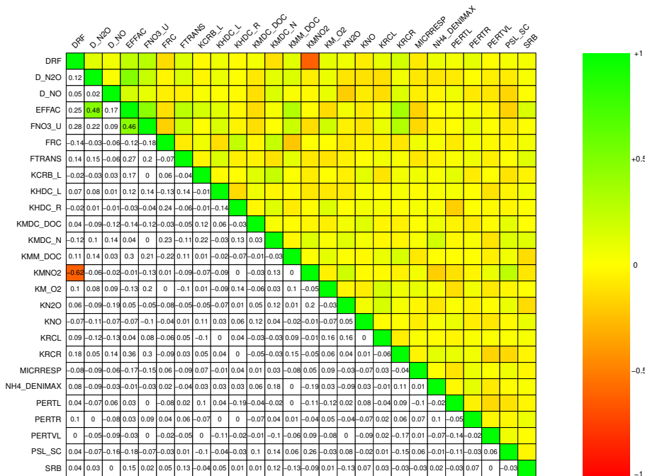
Fig. 8. Correlations of all 200 000 post burn-in parameter samples.
