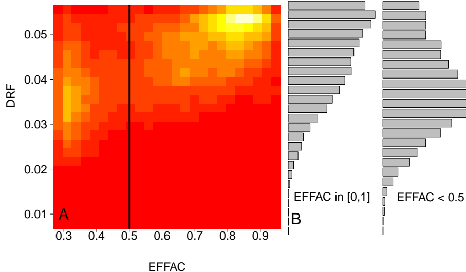
Fig. 2. A: Heat-map of 2-dimensional marginal distribution of EFFAC and DRF (decomposition rate factor), the brighter the polygons, the higher the posterior value. B: histogram of DRF using all values and histogram of DRF using only values of DRF, where EFFAC < 0.5.
