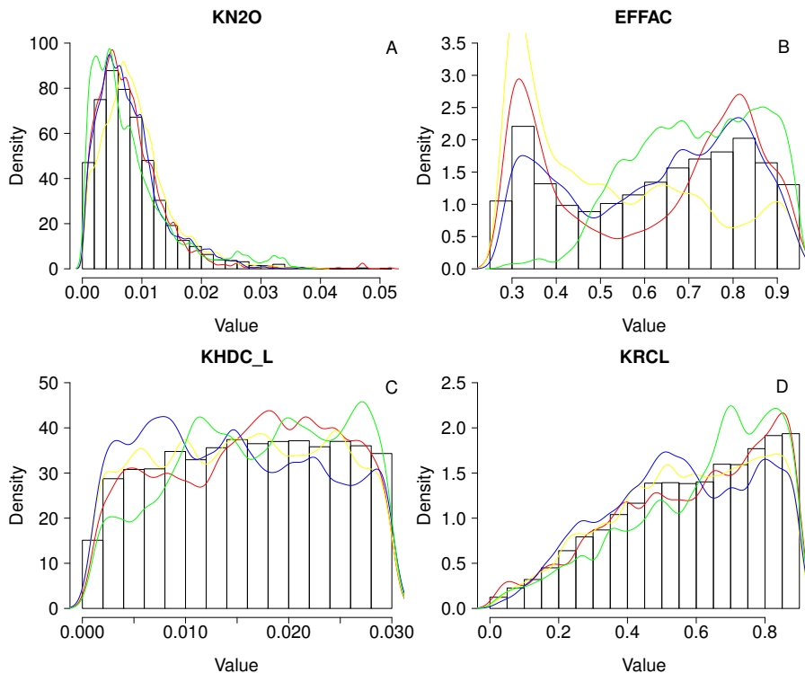
Fig. 4. Four typical histograms of marginal parameter distributions. The coloured density lines of a right-skewed (KN2O: loss rate of N 2 O during nitrification), bi-modal (EFFAC: describing the partitioning of CO 2 and DOC production during microbial decomposition of organic matter), flat (KHDC_L: decomposition constant of labile humads pool) and a left-skewed distribution (KRCL: decomposition constant of labile litter pool) were done by post burn-in samples of each individual chain, whereas the histograms are plotted using post burn-in samples of all chains.
