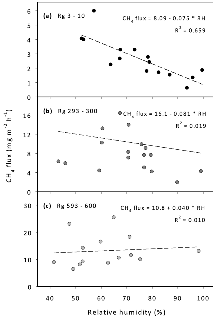
Figure 7: CH 4 flux plotted against relative humidity (RH). Data are selected by global radiation (R g ) in the range 3–10 W m -2 (a), 293–300 W m -2 (b) and 593–600 W m -2 (c). Only data with corresponding air temperature between 10 and 20 °C are displayed.
