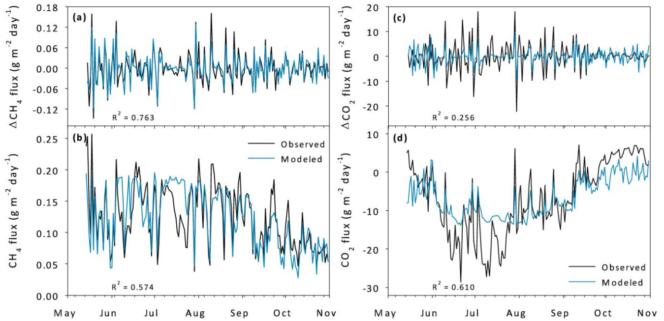
Figure 6: Observed and modeled daily fluxes of differenced data for \text{CH}_4 (a), original data for \text{CH}_4 (b), differenced data for \text{CO}_2 (c) and original data for \text{CO}_2 (d). The modeled data are created with an ARIMA(0,1,1) model, with R_g as explaining variable for \text{CH}_4 and R_g and T_{\text{soil}} for \text{CO}_2 . The error terms with the autoregressive part for the modeled data are not included in these graphs and in the coefficients of determination ( R^2 ).
