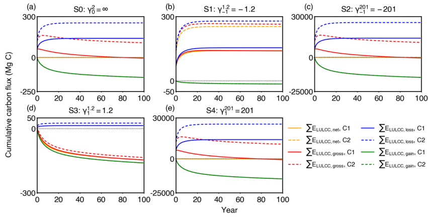
Figure 3 Cumulative carbon flux ( \sum E_{LULCC} ) after an initial forest area change at t = 0 followed by no change in forest area, for the different scenarios S0 to S4 in Table 1 with different net and gross initial forest area changes. The response curves used in those bookkeeping model simulations are C1 in solid lines (Table 2) with a secondary-to-secondary forest change at t = 0 , and a logarithmic biomass recovery curve with an asymptote, and C2 in the dashed lines (primary-to-secondary forest change at t = 0 and a logarithmic biomass recovery curve with an asymptote). The dotted line is the zero line. Positive value of carbon flux indicates carbon emission to the atmosphere.
