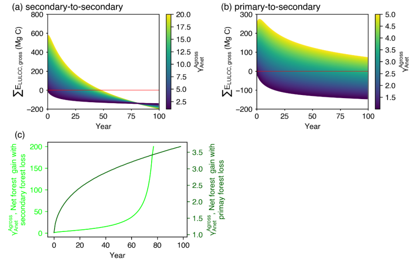
Figure 4 Time evolution of cumulative carbon flux ( \Sigma E_{LU,CC, gross} ) after an initial forest area change involving gross forest area changes followed by no forest area change. The three panels show results of our bookkeeping model for three case studies (a) a net forest gain at t = 0 with initial secondary forest loss followed by secondary forest regrowth (secondary-to-secondary, C1 in Table 2), (b) the same net area gain at t = 0 with initial primary forest loss followed by secondary forest regrowth (primary-to-secondary C2 in Table 2), and (c) the critical value of \gamma_{Anet}^{Agross} at which \Sigma E_{LU,CC, gross} is zero, going from a net source to a net sink for different time horizon in the x-axis. The colored curves in (a) and (b) have the same net area change ( A_{net} = +1 ha) at t = 0 but variable values of the initial gross-to-net area change ratios ( \gamma_{Anet}^{Agross} ). The red line in (a) and (b) is the zero line, defining the time after initial forest area change at which the system reaches a neutral carbon balance. The light and dark green lines in (c) represent the critical ratios for a net initial forest gain scenario with secondary-to-secondary (a) and primary-to-secondary (b) gross forest area change, respectively. Values larger than this critical value indicate that the initial forest area change has the net effect to emit CO_2 for a given time horizon in the x-axis. Exponential curve from Hansis et al. (2015) for carbon loss in all pools and gain in soil pool and logarithmic curve from Poorter et al. (2016) for gain in biomass pool are used in this example (Table 2).
