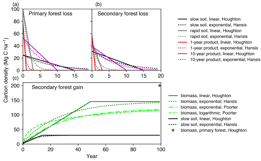
Figure 1 Response curves for tropical moist forest in bookkeeping models and from a recent field study. Solid and dotted lines indicate the linear (Houghton, 1999) and exponential (Hansis et al., 2015) curves, respectively. Lime dashed and dash-dotted lines are the logarithmic and exponential curves from forest plots (Poorter et al., 2016). Vegetation carbon density in primary forest (Houghton, 1999) is also shown as a star in (c) for comparison.
