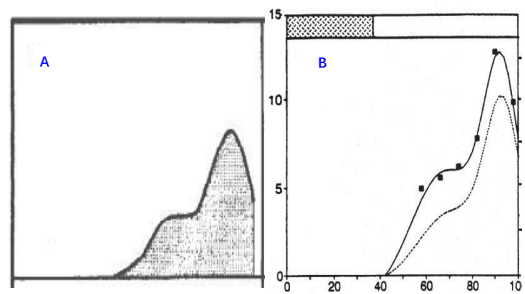
Radius of stem of Pinus sylvestris (relative)
