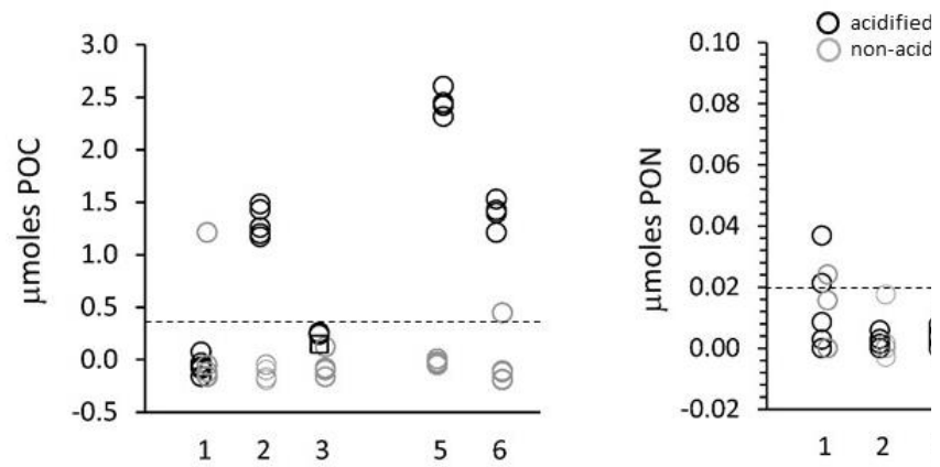
Figure 3. The effect of vapor acidification on POC and PON using precombusted GFF filters with distilled water. Five experiments using five samples each for acid treatment and blanks. Fresh concentration except where noted. 1. The desiccator was cleaned with solvent; 2. Desiccator was cleaned with distilled water; 3. Desiccator cleaned with solvent. The desiccator top was sealed with grease in 5 and 6. In each experiment, one acid-treated sample is marked as a square because we applied half of the concentration of two duplicate samples. The dashed line indicates the lower limit of detection.
