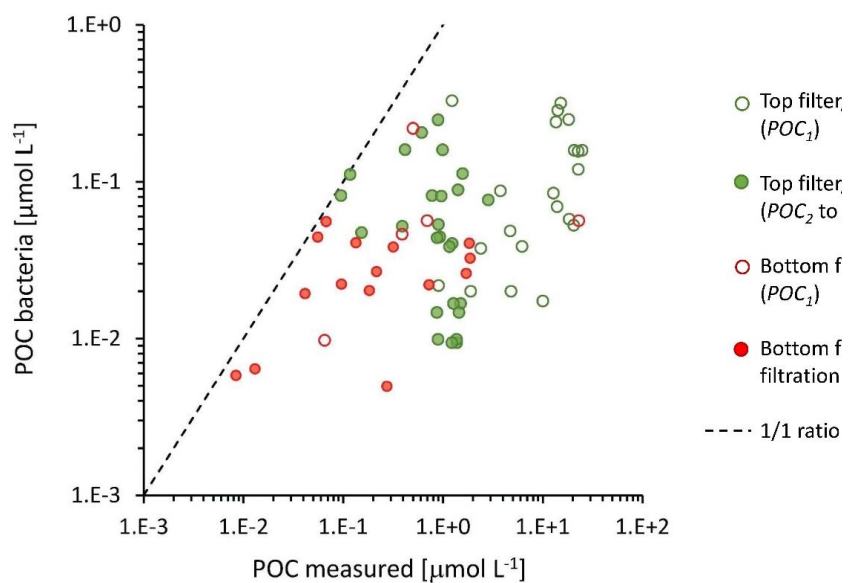
Figure 8. Measured POC versus the POC calculated to represent the bacterial biomass retained. Bacterial POC was calculated from bacterial abundance of the sample and a retention efficiency per passage.
