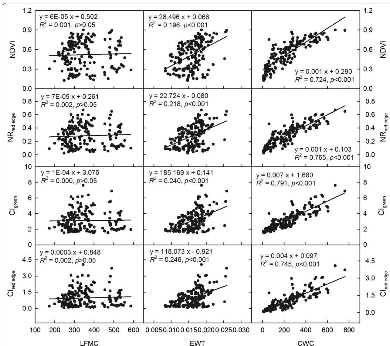
Fig. 3 Correlation analysis of hyperspectral vegetation indices, normalized difference vegetation index (NDVI), red edge normalized ratio (NR red edge ), green chlorophyll index (Cl green ), and red edge chlorophyll index (Cl red edge ) vs. canopy water content (CWC, g m -2 ), leaf equivalent water thickness (EWT, g cm -2 ), and live fuel moisture content (LFMC, g cm -2 ) for maize during the growing seasons from 2013 to 2015
