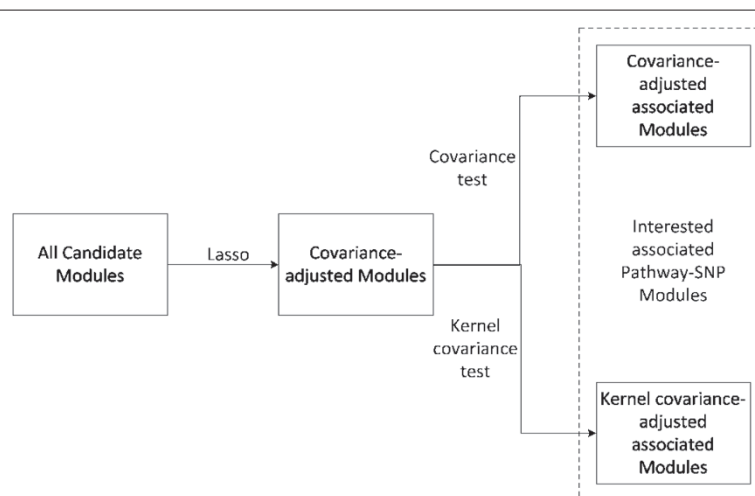
Fig. 1 Flowchart of our strategy. Flowchart of our strategy for detecting pathway-associated SNP. We first perform Lasso to adjust the effects of SNPs on the means of gene expression. Then we use covariance test and kernel covariance test to select candidate pathway-SNP modules
