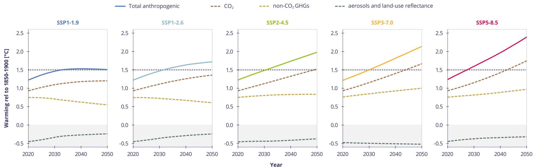
FIGURE 1: Warming contributions relative to pre-industrial levels (1850-1900) from groups of anthropogenic drivers, i.e. CO 2 , non-CO 2 greenhouse gases including CH 4 , aerosols and land-use reflectance, for all five illustrative emissions scenarios assessed by IPCC AR6 WGI for 2020-2050. Only central estimates are provided here for clarity.
