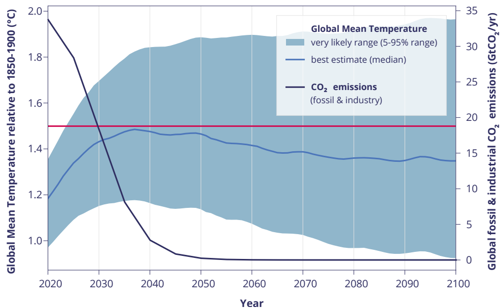
FIGURE 3: Annual fossil & industrial CO 2 emissions and projected global mean temperature trajectory, central estimate and very likely (5-95% model) range, relative to pre-industrial levels (1850-1900) of the original MAGICC7 climate emulator experiment before changing the model ECS and aerosol forcing by \pm 10\% and switching off permafrost feedbacks. Model setup and emissions scenario specifics are based on Nicholls (2021) 17 .
