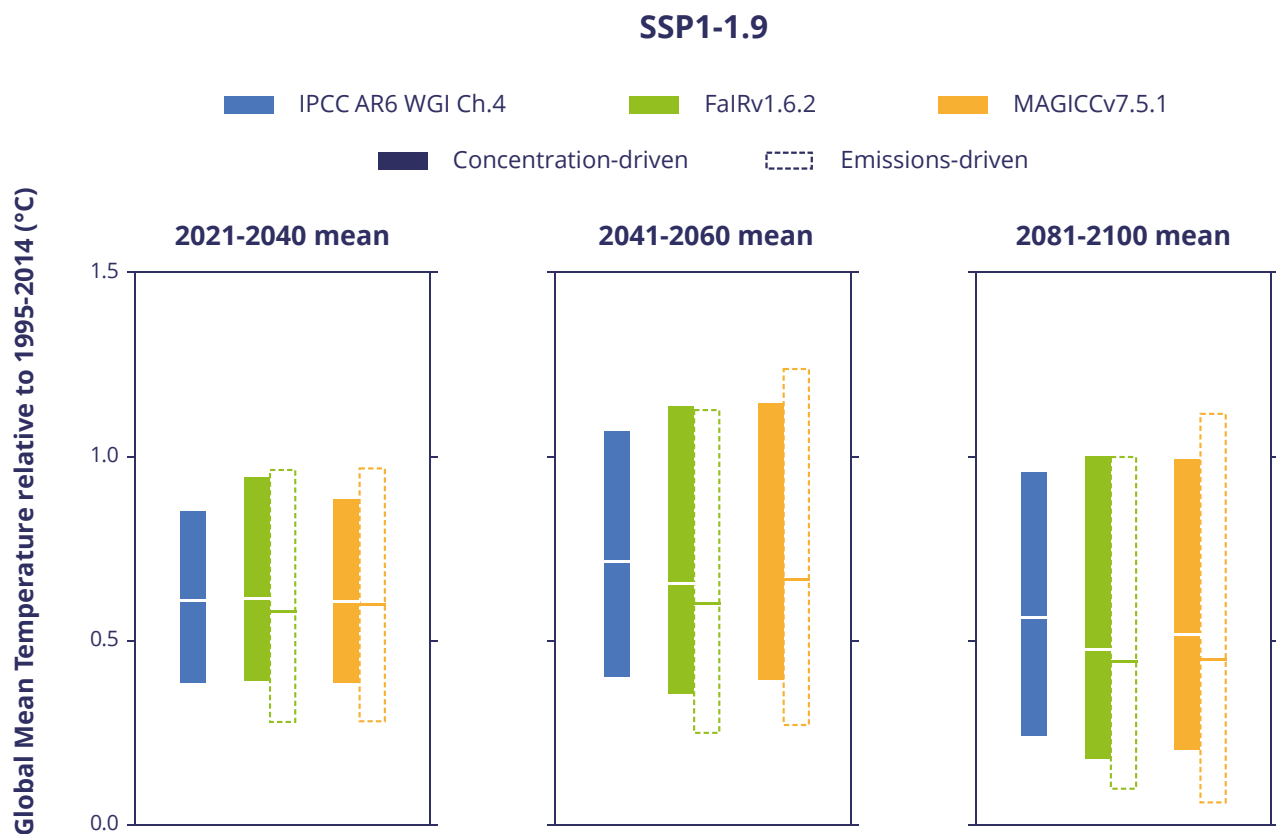
FIGURE 5: Comparison of 21 st century global mean temperature change for concentration- and emissions-driven emulator runs under the same very low emissions scenario (SSP1-1.9). Central estimates and very likely (5-95% model) ranges are provided for the near-term (2021-2040), mid-term (2041-2060), and long-term (2081-2100) relative to the recent reference period 1995-2014. The IPCC AR6 WGI Chapter 4 assessment as well as concentration-driven estimates shown in darker shading, emissions-driven estimates in lighter shading. Figure based on IPCC AR6 WGI Cross-Chapter Box 7.1 Figure 1.
