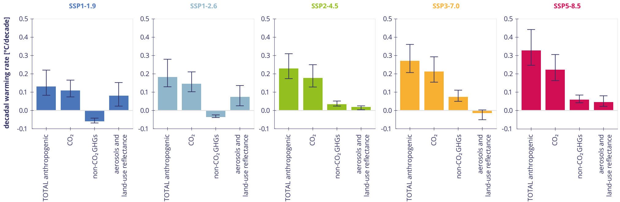
FIGURE 2: Average decadal warming rates over the next 20 years (2021-2040) by groups of anthropogenic drivers, i.e. CO 2 , non-CO 2 greenhouse gases including CH 4 , aerosols and land-use reflectance, for all five illustrative emissions scenarios assessed by IPCC AR6 WGI. Bars represent the central estimates, whiskers (dark blue) show the very likely (5-95% model) range.
