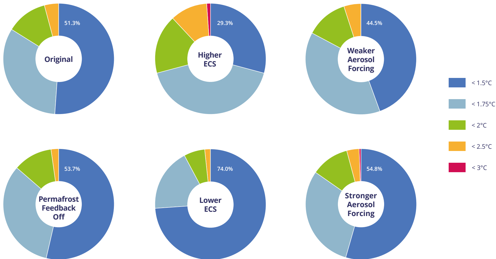
FIGURE 4: “Climate wheels” showing the probabilities of staying below 1.5°C, 1.75°C, 2°C, 2.5°C, and 3°C in the 21 st century for the different MAGICC7 experiments ( \pm 10\% Equilibrium Climate Sensitivity (ECS), \pm 10\% aerosol forcing strength, permafrost off) under the same stringent emissions reduction pathway that reaches zero fossil and industrial CO 2 emissions around 2050.
