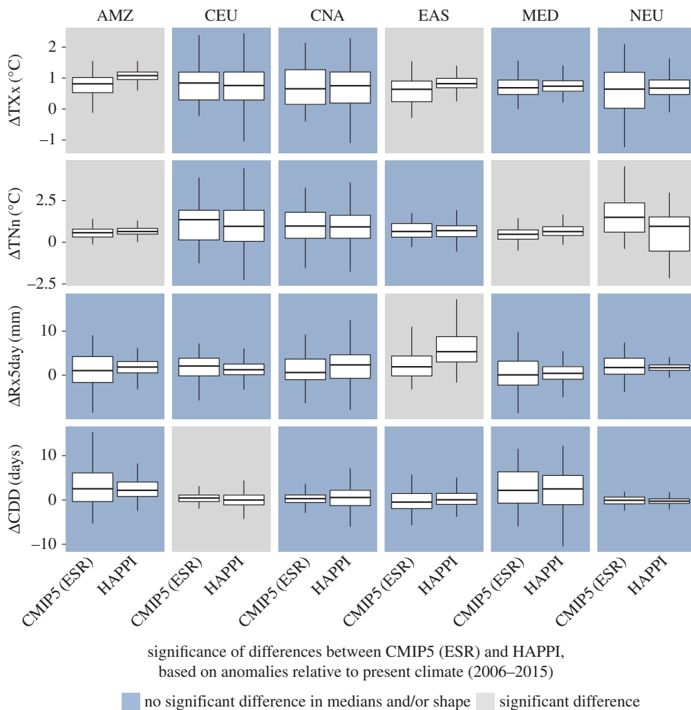
Figure 3. Changes in regional extremes at 1.5°C of global warming estimated from the ESR approach based on CMIP5 simulations ('CMIP5 (ESR)') based on [5,8], and from the HAPPI simulations. The changes are computed with respect to present-day climate (1°C of warming for ESR-CMIP5, respectively 2006–2015 in HAPPI). Displayed are box plots indicating the median (middle horizontal line), interquartile range (25th and 75th percentile) indicated with lower (25th percentile) and upper (75th percentile) hinges of the box, and whiskers extending to the lowest (highest) value that is within 1.5 times the interquartile range of the upper (lower) hinge (for figures including outliers, see electronic supplementary material). Analyses are provided for changes in maximum daytime temperature (TXx), minimum night-time temperature (TNn), annual maximum consecutive 5-day precipitation (Rx5day) and consecutive dry days (CDD), and for six regions (figure 2) as defined in the IPCC SREX report [33]: AMZ (Amazon), CEU (Central Europe), CNA (Central North America), EAS (Eastern Asia), MED (Mediterranean) and NEU (Northern Europe). Blue background shading indicates when there is no significant difference in the median or the shape between the ESR-CMIP5 and HAPPI estimates (based on Wilcoxon rank-sum test). (Online version in colour.)
