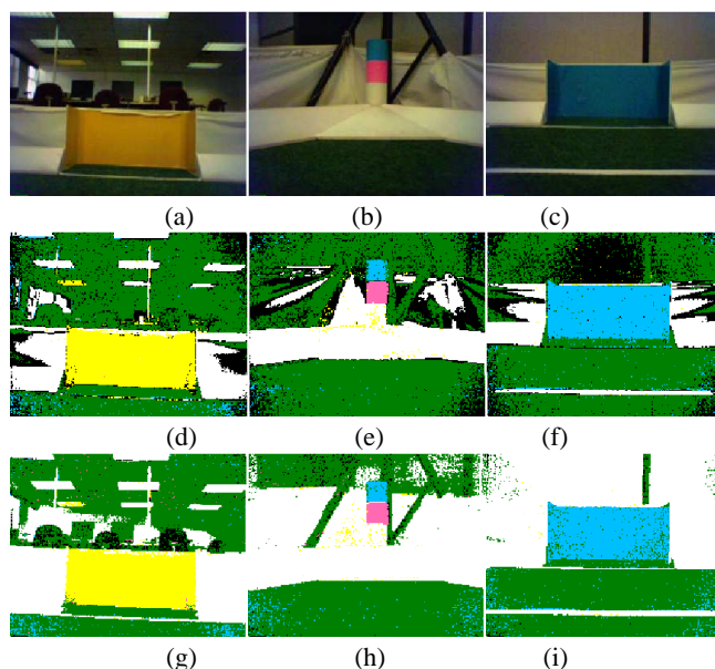
Figure 4: Sample Images without ball. (a)-(c) Original Images, (d)-(f) YCbCr color space, (g)-(i) LAB color space
