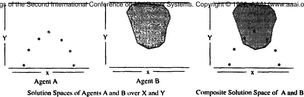
Figure 1: Local and Composite Search Spaces
