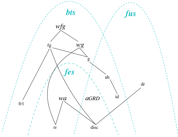
Figure 1: Inclusions between decidable cases
