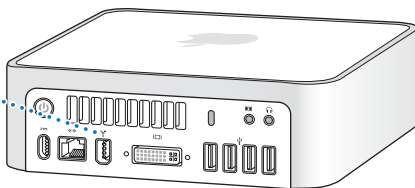
FireWire 400 port
