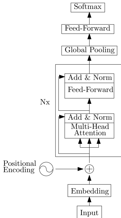
Fig. 1: The Transformer Encoders system for IroSvA19.
