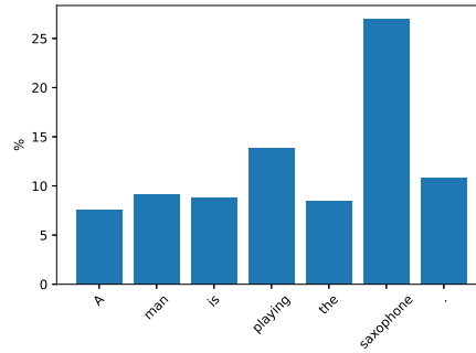
Figure 2: Example of word importance.
