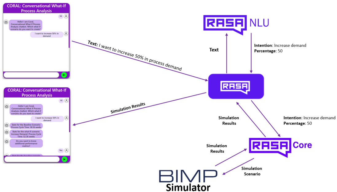
Figure 1: Coral's implementation architecture.
