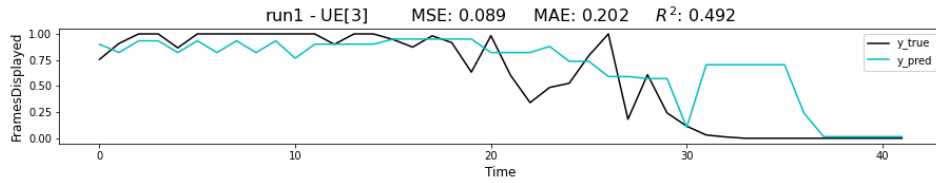
(b) RT-prequential
