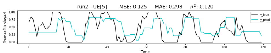
(a) HRT-hold-out
