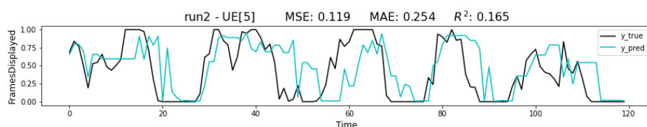
(b) RT-hold-out
