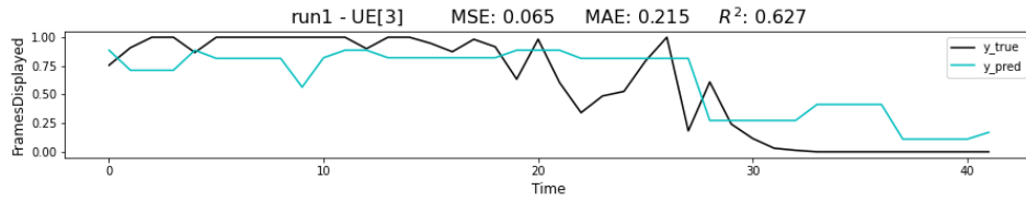
(a) HRT-prequential
