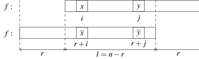
Figure 1: The word f and its 2-error overlap of length l
