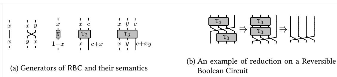
Figure 1: Generators of Reversible Boolean Circuits and a reduction on them
