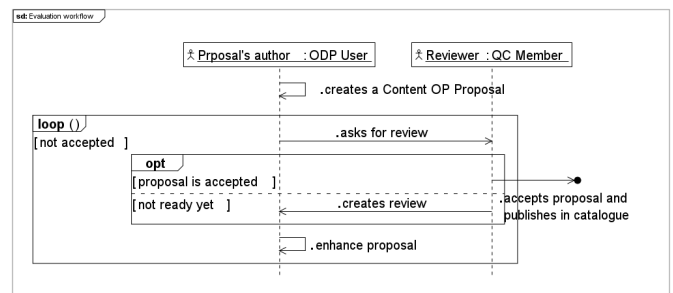
Figure 1: Evaluation example
