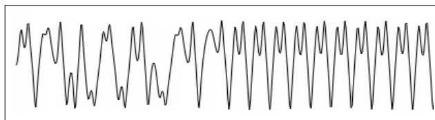
Figure 1. DoubleWell oscillator with F = 0.4 , w = 1 , \delta = 0.25 .
