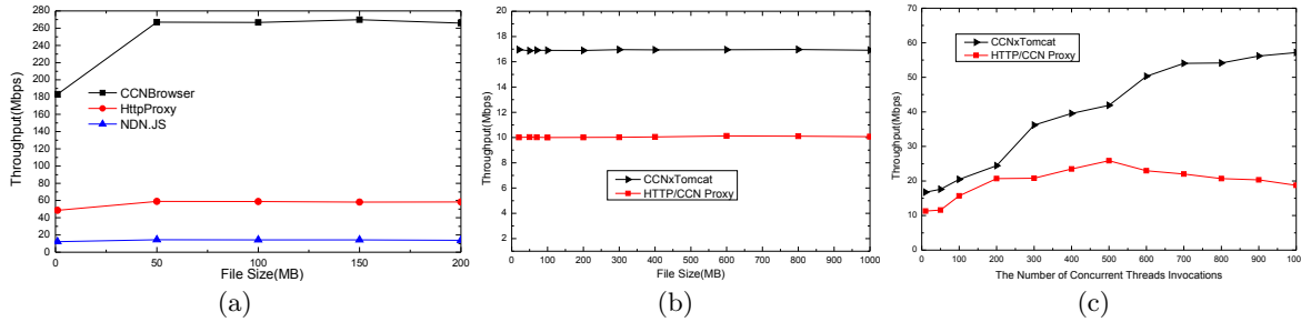
Figure 3: Test results: (a) CCNBrower vs. NDN.JS and HTTP/CCN Proxy in terms of the single file test. (b) CCNxTomcat vs. HTTP/CCN Proxy in terms of the single file test. (c) CCNxTomcat vs. HTTP/CCN Proxy in terms of the throughput.
