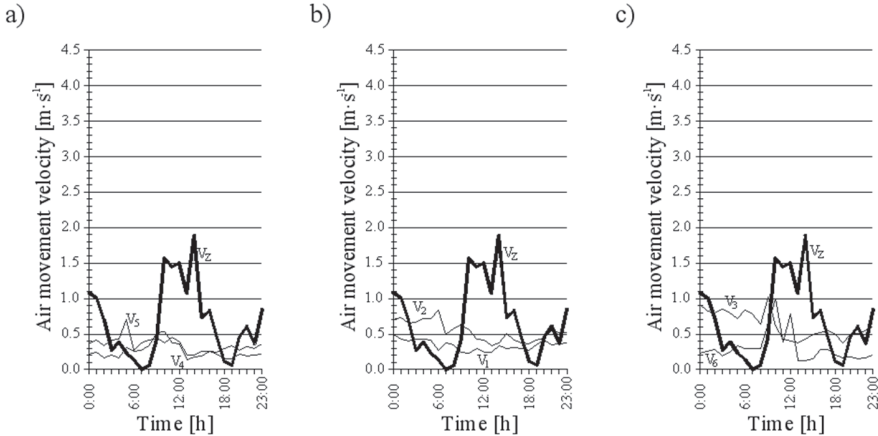
Figure 5. Wind velocity ( V_z ) and air movement velocity ( V_{1-6} ) in particular measurement points on 4 February 2012 inside the barn in Kobylany for three technological groups; a) group 1, b) group 2, c) group 3 (own source)
