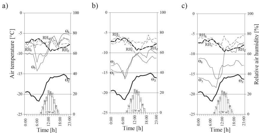
Figure 4. Temperature ( \Theta_z , \Theta_{1-6} ), relative air humidity ( RH_2 , RH_{1-6} ) and solar radiation intensity ( I ) on a cloudy day of 4 February 2012 inside the barn in Kobylny for three technological groups; a) group 1, b) group 2, c) group 3 (own source)
