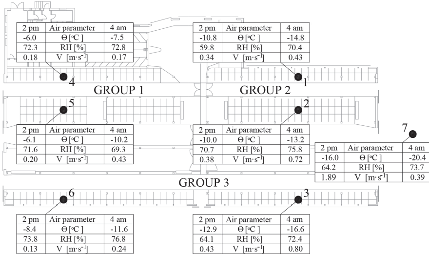
Figure 7. Layout of the building with measurement points (1–7) and hourly average values registered on 4 February 2012 at 4 am and 2 pm (own source)
