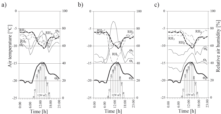
Figure 2. Temperature ( \Theta_z , \Theta_{1-6} ), relative air humidity ( \text{RH}_z , \text{RH}_{1-6} ) and radiation intensity observations (I) on a sunny day of 3 February 2012 inside the barn in Kobylany; a) group 1, b) group 2, c) group 3 (own source)
