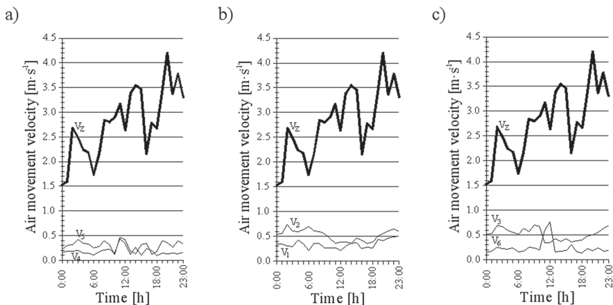
Figure 6. Wind velocity ( V_z ) and air movement velocity ( V_{1-6} ) in particular measurement points on 7 February 2012 inside the barn in Kobylany for three technological groups; a) group 1, b) group 2, c) group 3 (own source)
