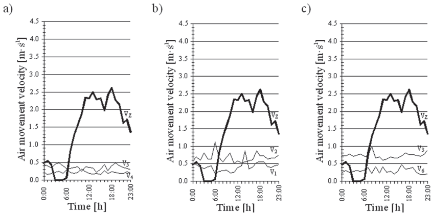
Figure 3. Wind velocity measurements ( V_z ) and air movement measurements ( V_{1-6} ) in particular measurement points on 3 February 2012 inside the barn in Kobylny for three technological groups; a) group 1, b) group 2, c) group 3, V_z – wind velocity, V_{1-6} – air movement velocity (own source)
