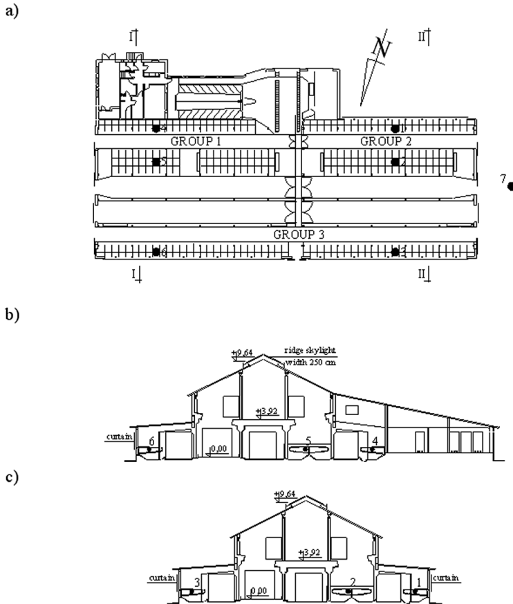
Figure 1. Location of measurement points: temperature, relative air humidity and air movement; a) horizontal projection, b) cross-section I-I, c) cross-section II-II, 1-7 – measurement points (own source)
