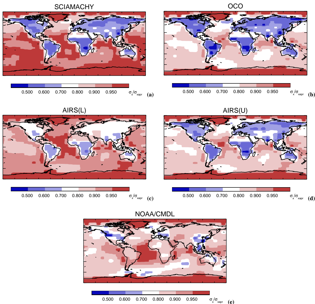
Fig. 2. Fractional change in flux uncertainty ( \sigma_x/\sigma_{xpr} ) per year and per model grid cell gained by inversions on the basis of measurements by (a) SCIAMACHY; (b) OCO; (c) AIRS(L); (d) AIRS(U) (e) NOAA/CMDL, for process weighted and space correlated (PW/SC) prior uncertainties (see text).
