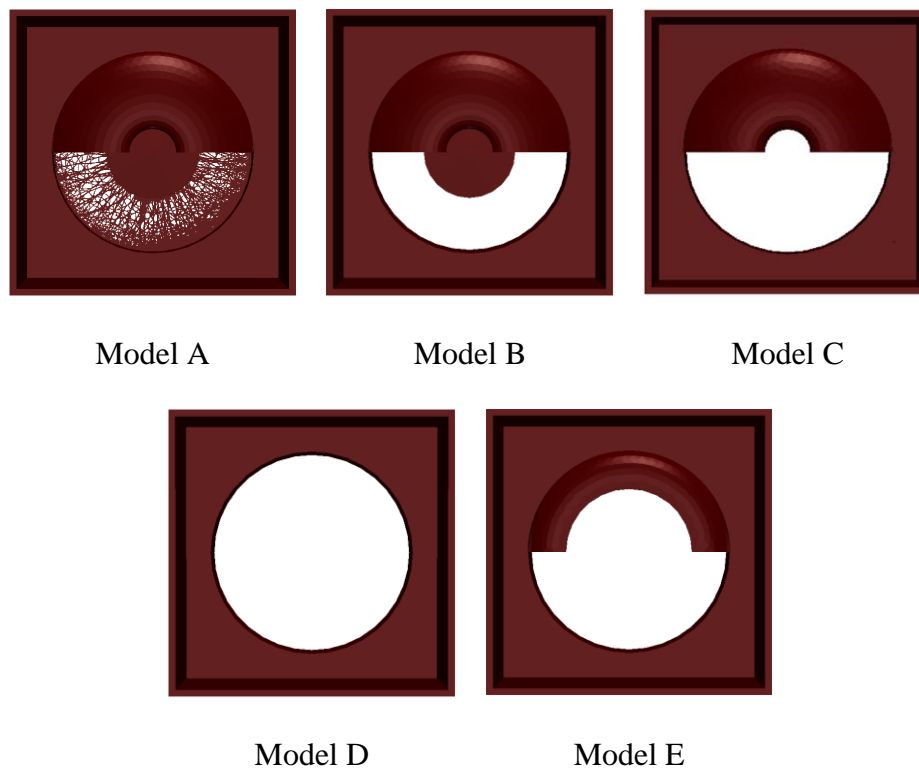
Fig. 4.3 The different models used in LBM simulations. Borders have been partially removed for illustrative purposes. Model A is the full model with borders, margo, and torus. Models B-D have had the margo, torus, and borders, respectively, removed to assess individual resistances relative to Model A. Model E represents a pit that has undergone steam explosion in which parts of the structure have been removed and the borders have detached somewhat.
