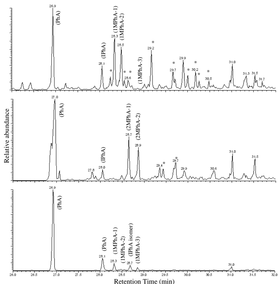
Fig. 2. The relative abundance vs. retention times are presented for the GC-MS chromatograms of the TMS-derivatives of phthalic acid (PhA), isophthalic acid (IPhA), 1-methylphthalic acid (1MPhA-1 to -3) and 2-methylphthalic acid (2MPhA-1 to -2) isomers from the photooxidation of 1-MN (top: absence of \text{NO}_x , bottom: presence of \text{NO}_x ) and 2-MN (middle: absence of \text{NO}_x ) from ER467, ER470, and ER468, respectively. The peaks are scaled using the M-15 peak ( m/z 295 for PA and m/z 309 for 1MPhA-1 to -3 and 2MPhA-1 to -2). For the experiments in the presence of \text{NO}_x the ratio of the \Sigma MPhA to PhA is considerably lower using the ion scaling shown here. (*) represent peaks having similar mass spectra as 1MPhA or 2MPhA.
