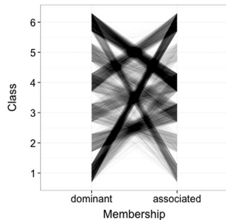
Fig. 6. Associations between the six different spectral classes derived by classifying the scores from the principal component analysis of the global spectra with the fuzzy-c-means algorithm.
