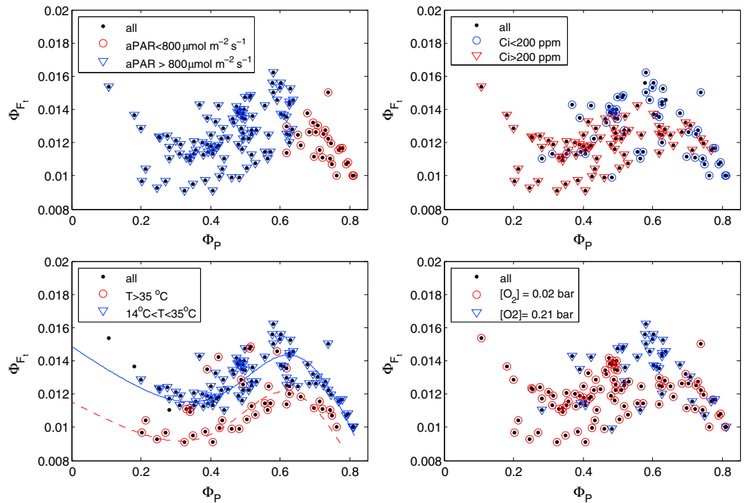
Figure 3. The data and model results of the cotton experiment presented as \Phi_{F_i} versus \Phi_P , with different symbols for driving variables. The lines are computed from the empirical K_N(x) with temperature correction for 25°C (solid line) and 35°C (dashed line).
