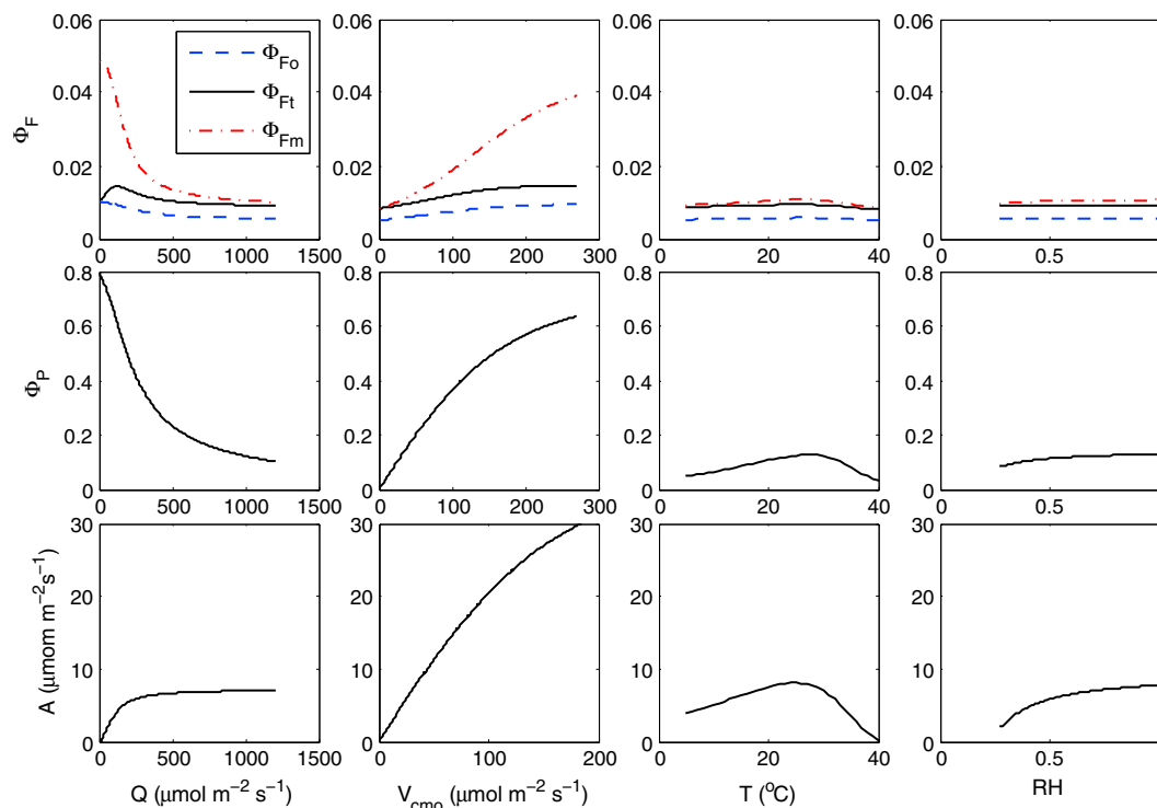
Figure 11. One-by-one sensitivity analysis of the modeled yields (fluorescence and photochemistry) and photosynthesis of a “standard” leaf to four input variables. The sensitivity was calculated for drought relation between x and K_N . The parameters of the standard leaf were leaf boundary [\text{CO}_2] = 380 \text{ ppm} , a\text{PAR} = 1000 \mu\text{mol m}^{-2}\text{s}^{-1} , leaf temperature T = 20^\circ\text{C} , relative humidity \text{RH} = 70\% , V_{\text{cmo}} = 30 \mu\text{mol m}^{-2} \text{s}^{-1} , and Ball-Berry stomatal conductance parameter m = 8 .
