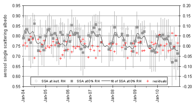
Figure 6. Variations in the aerosol single scattering albedo at 550 nm at IPR: monthly mean values at instrumental RH (open circles), at 0 % RH (squares), least mean square fit of the monthly mean values at 0 % RH (line), and residuals (crosses, right axis). Error bars show the standard deviation of the monthly mean values at 0 % RH.
