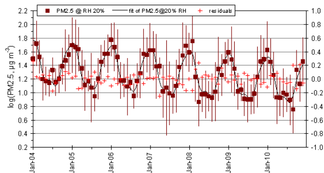
Figure 1. Variations in \text{PM}_{2.5} at IPR: logarithm of the monthly mean values (squares), least mean square fit (line), and residuals (crosses, right axis). Error bars show the standard deviation of the log of the monthly averages.
