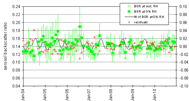
Figure 5. Variations in the aerosol backscatter ratio at 550 nm at IPR: monthly mean values at instrumental RH (open circles), at 0 % RH (squares), least mean square fit of the monthly mean values at 0 % RH (line), and residuals (crosses, right axis). Error bars show the standard deviation of the monthly mean values at 0 % RH.
