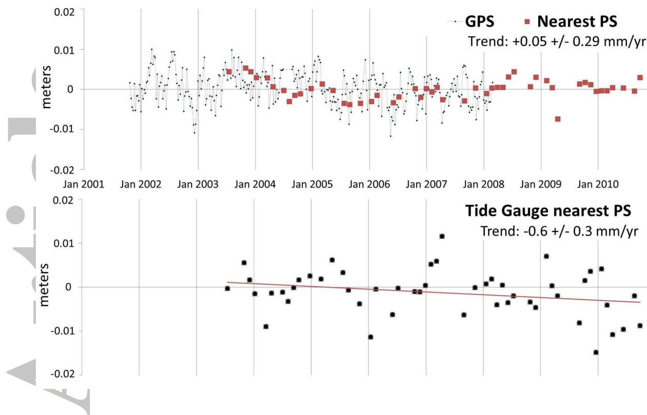
Figure 2. PSI and GPS time series projected along the satellite line of sight with (a) the persistent scatterer nearest to the continuous GPS antenna; and (b) the persistent scatterer nearest to the tide gauge. The red line shows the best linear fit.
