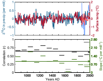
4. Antarctic Peninsula
