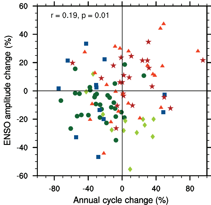
(a) ENSO amplitude vs. annual cycle change
