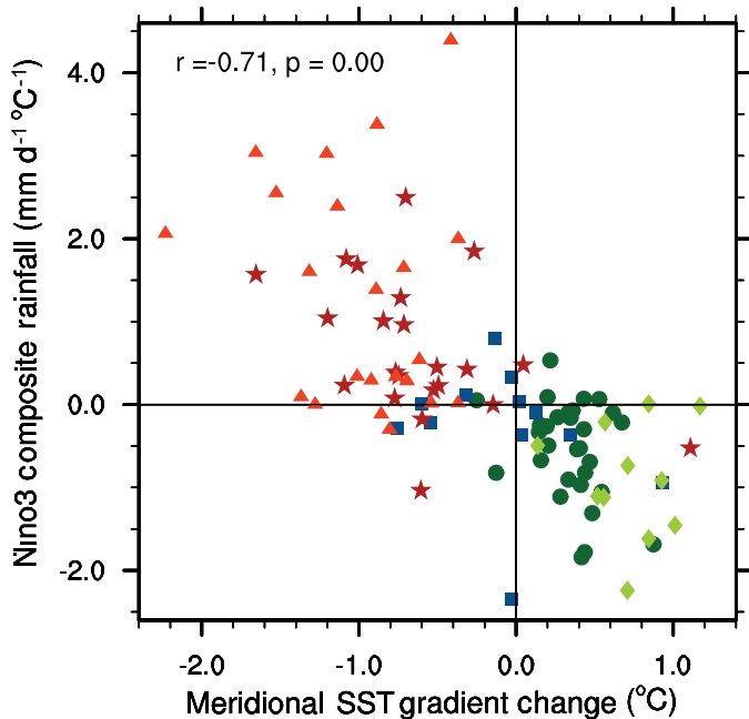
(c) NINO3 rainfall vs. meridional SST gradient
