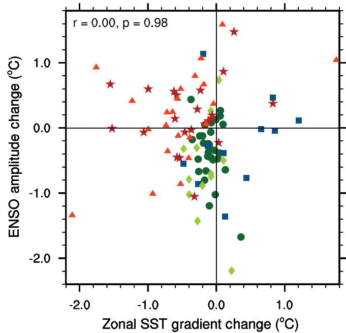
(b) ENSO amplitude vs. zonal SST gradient change
