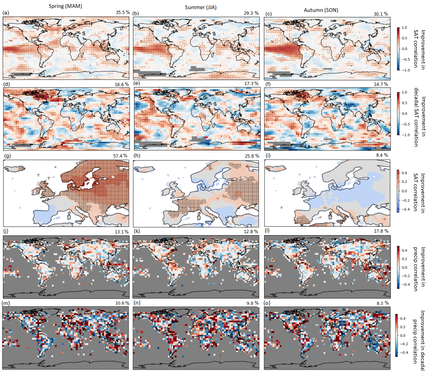
Figure S9 – Improvement in correlation in Boreal spring (mam), summer (jja) and autumn (son). All panels the same as figure 6 but for different seasonal means.
