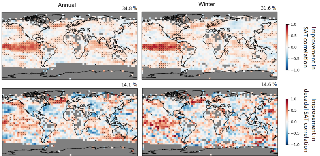
Figure S8 – Improvement in annual and winter (djf) correlation between temperature in observations and assimilated model (with the forcing removed). Same as figure 6a-d except the correlations have been calculated against a version of HadCRUT5 with no infilling.
