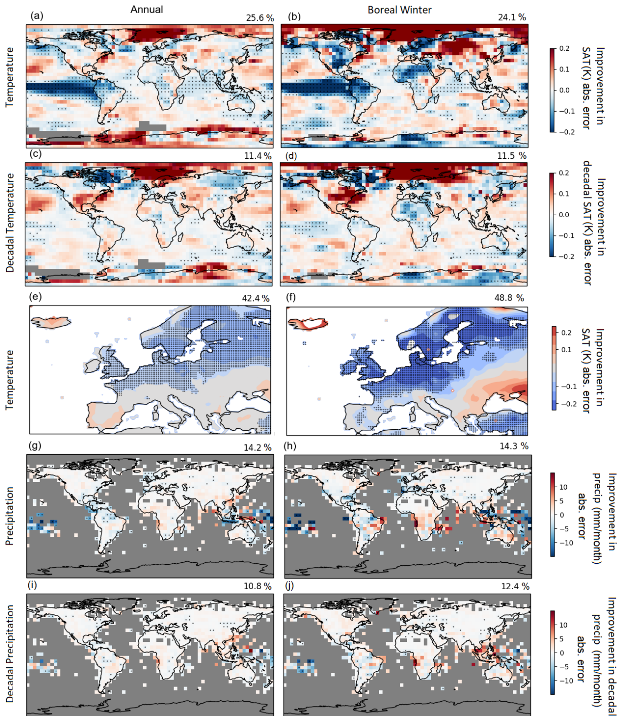
Figure S10 – Improvement in absolute mean error in annual and Boreal winter (djf). All panels the same as figure 6 except that the panels show bias calculated as difference in absolute mean error.
