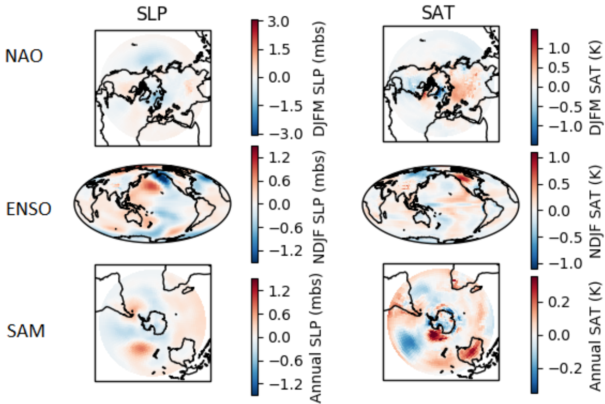
50 Figure S5 – Difference in the regression patterns between observations and observed index and model and observed index. From top to bottom: NAO, ENSO, SAM, difference in the regression between the observed index and the observed spatial pattern of sea level pressure (from 20CRv3 Slivinski et al. 2021) and surface air temperature (from HadCRUT5; Morice et al. 2021) the regression between the observed index and the DA model spatial pattern (Difference between left and middle column Fig 4 and Fig 5).
