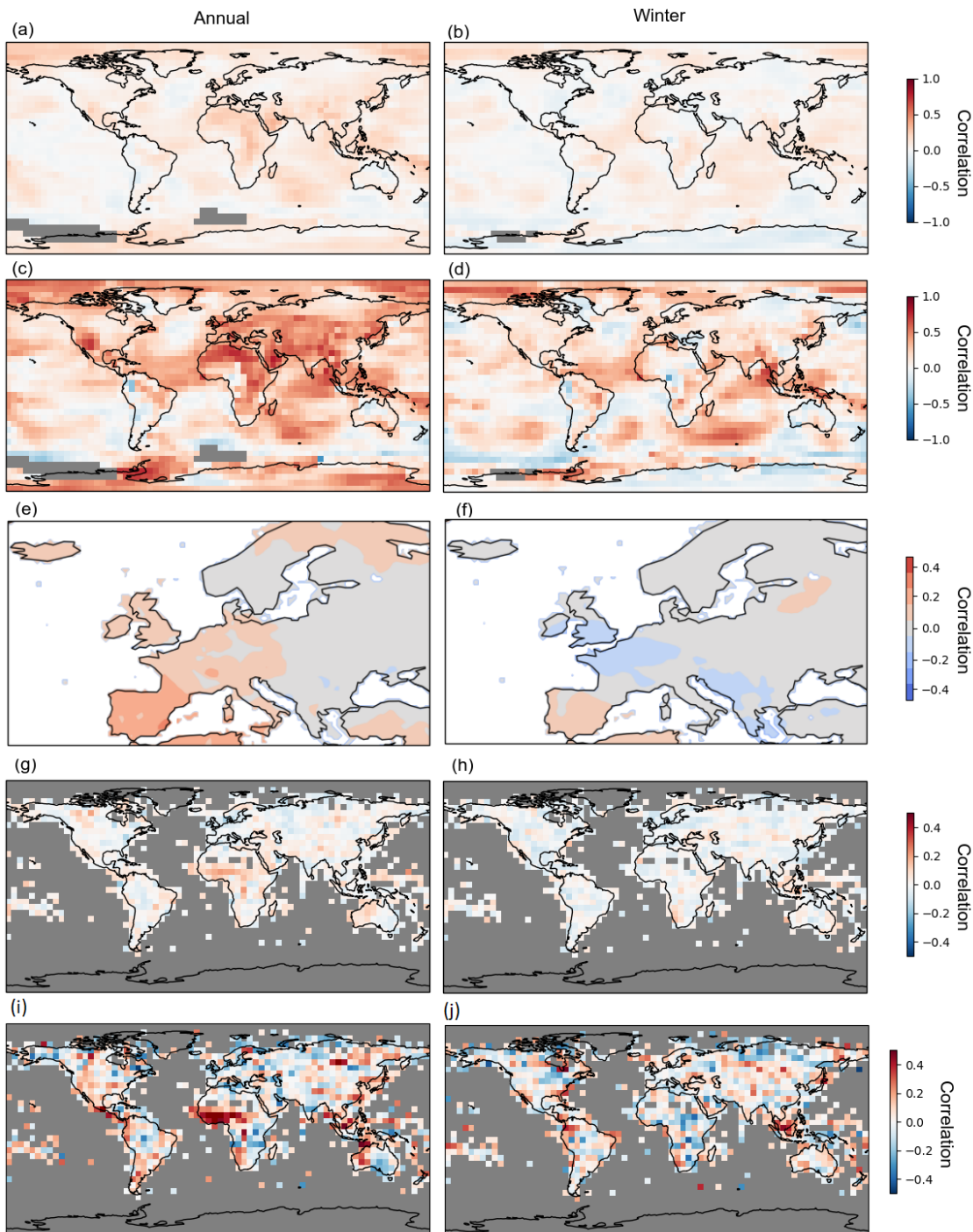
60 Figure S7 – Annual and winter (dJF) mean correlation between temperature in observations and a weighted mean of forcing-only model simulations (with no assimilation). As in figure 6 but correlations given as the raw correlations between the weighted ensemble mean of the forcing-only simulations and observations, i.e. results show the forced component.
