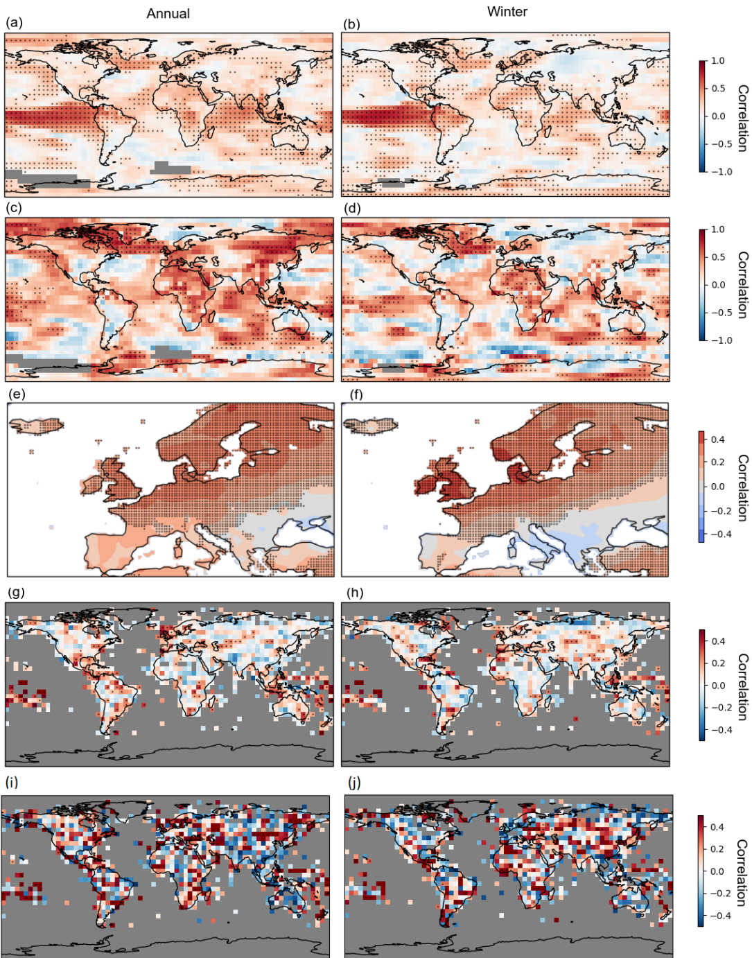
Figure S6 – Annual and winter (djf) correlation between temperature in observations and assimilated model. As in 55 figure 6 but correlations given as the raw correlations between assimilated model and observations rather than the improvement in correlation (with the correlation of the forced component removed).
