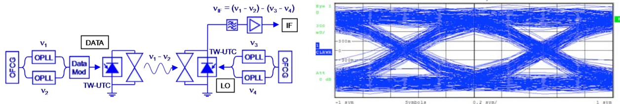
Fig. 2. THz communications system employing a UTC optoelectronic mixer for heterodyne detection and received 500 kb/s BPSK eye diagram from 80 GHz communication link using heterodyne receiver.
