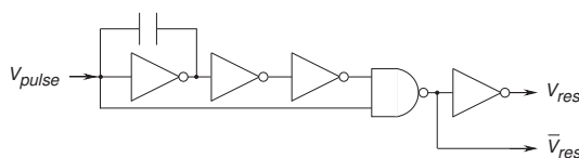
Fig. 6. Schematic of the delay-and-inverter circuit.
