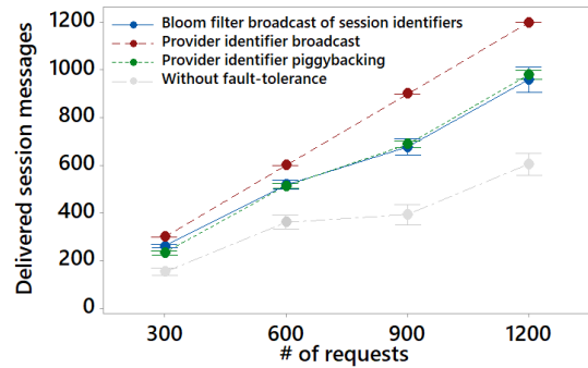
Figure 7: Delivered session messages for the three fault-tolerant mechanisms and the session mechanism without fault-tolerance for the four evaluation setups.
