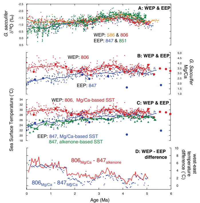
Figure 4. (A) Planktonic ( G. sacculifer without sac-like final chamber) foraminifera \delta^{18}\text{O} records from two western equatorial Pacific (WEP) locations: Deep Sea Drilling Project site 586 (orange) (Whitman and Berger, 1992) and Ocean Drilling Project (ODP) site 806 (red) (Chaisson and Ravelo, 2000; Wara et al., 2005) and two eastern equatorial Pacific (EEP) locations: ODP site 847 (blue) (Chaisson and Ravelo, 2000; Wara et al., 2005) and ODP site 851 (Cannariato and Ravelo, 1997). (B) Planktonic ( G. sacculifer without sac-like final chamber) foraminifera Mg/Ca records from the western equatorial Pacific location, ODP site 806 (red), and eastern equatorial Pacific location, ODP site 847 (blue). Small dots and smoothed line are data from Wara et al. (2005); large dots are data from Rickaby and Halloran (2005). (C) Sea surface temperature (SST) ( ^\circ\text{C} ) estimates for the western equatorial Pacific site 806 (red) and eastern equatorial Pacific site 847 (blue) based on Mg/Ca records (shown in B) using Dekens et al. (2002) calibration and for the eastern equatorial Pacific site 847 (green) based on \text{U}^{13}\text{C} measurements (this study). (D) The west minus east SST difference record calculated by subtracting the site 847 Mg/Ca-based SST record from the site 806 Mg/Ca-based SST record (blue) (adapted from Wara et al., 2005) and by subtracting the site 847 alkenone-based SST record from the site 806 Mg/Ca-based SST record (red).
