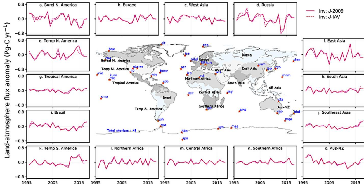
Figure S1: Regional CO 2 fluxes anomalies, similar to Fig. 6, for showing the effect of inter-annually varying \mathbf{J} -matrix (J-IAV) vs annually repeating \mathbf{J} -matrix corresponding to the year 2009 (J-2009). This checking was conducted using the inversion results submitted to GCP-2018 budget (Le Quéré et al., 2018). Please note that the PFU, MDU and other model setups were differently set at that time and the flux results cannot be compared with those in the present study.
