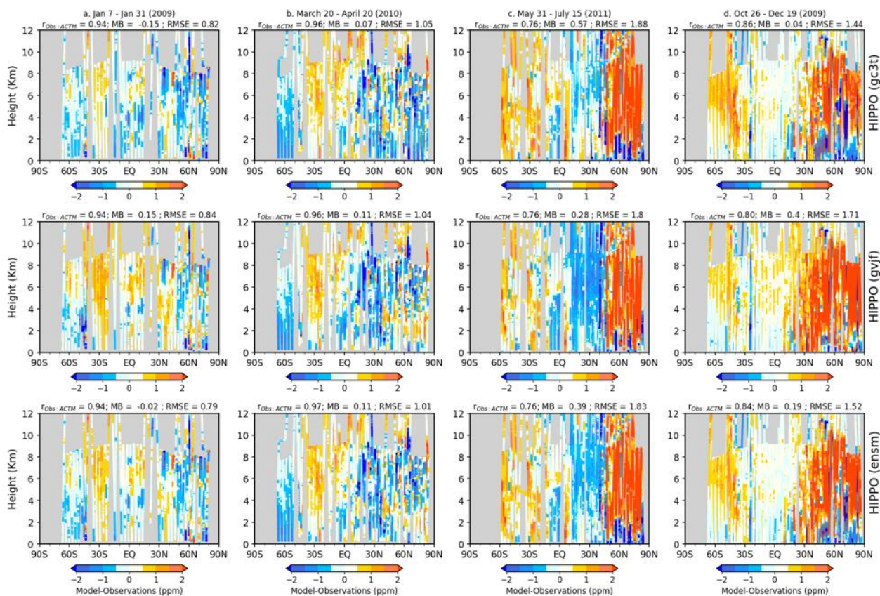
Figure S5: Mismatch between simulated and measured CO 2 during HIPPO aircraft campaigns. The observed and modelled data are binned and averaged at intervals of 2.5° latitude and 500-meter altitude. The grey area shows no flights at those altitudes and altitudes. Modelled mole fractions were simulated from the three posterior flux cases. The upper, middle, and the bottom row show simulations for “gc3t”, “gvjf”, and “ensm” cases, respectively. The correlation coefficients ( r ), mean bias (MB), and root-mean-square error between observations and simulations are also shown in the title.
