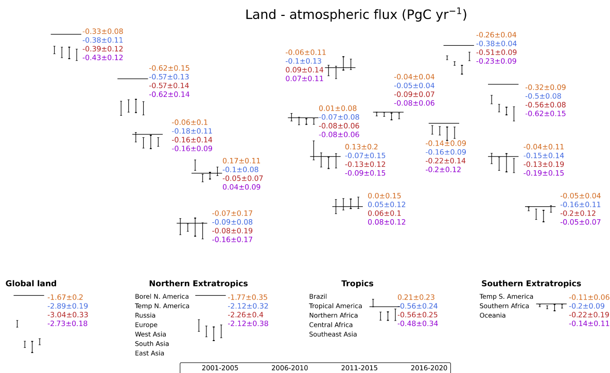
Fig S3. Mean CO 2 fluxes and spread ( \pm 1\sigma ) among 16 inversion cases over global, three aggregated latitudinal bands and 15 aggregated land regions. The bars in the down-facing directions represent carbon sinks, whereas the bars in the upward-facing directions represent carbon source.
