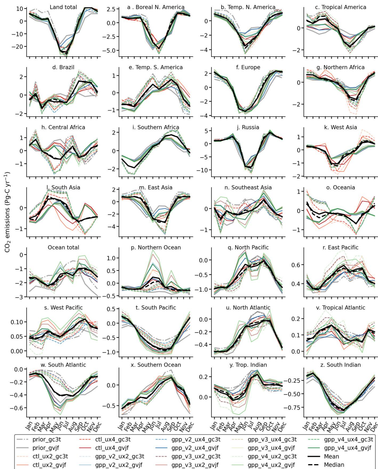
Figure S2. Seasonal variations in monthly-mean CO 2 fluxes at regional scales over 15 land (upper 4 rows) and 11 ocean (lower 3 rows) regions, along with global land and ocean totals. Note that all panels use different y-scale. The seasonal cycles only over a few (ill-constrained) regions are significantly corrected by inversions.
