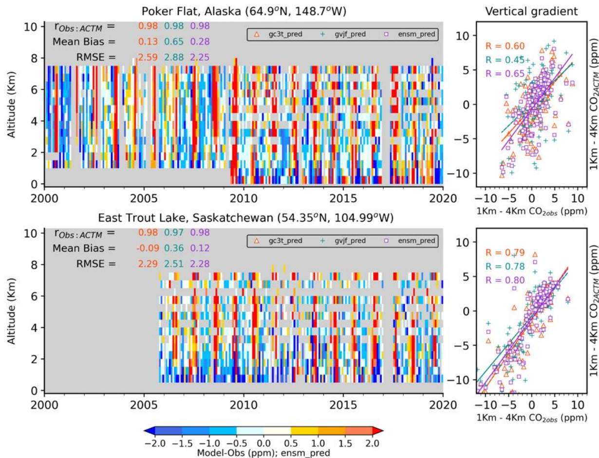
Figure S8. Validation of simulated CO 2 mixing ratios using regular NOAA aircraft profiles over two sites located in boreal North America (see also Figure xx for the location of profiles). The left panel shows the bias (model minus observations) as a function of altitude, and the right panel shows the scatter plot between the observed and modelled vertical gradient using three prescribed emissions.
