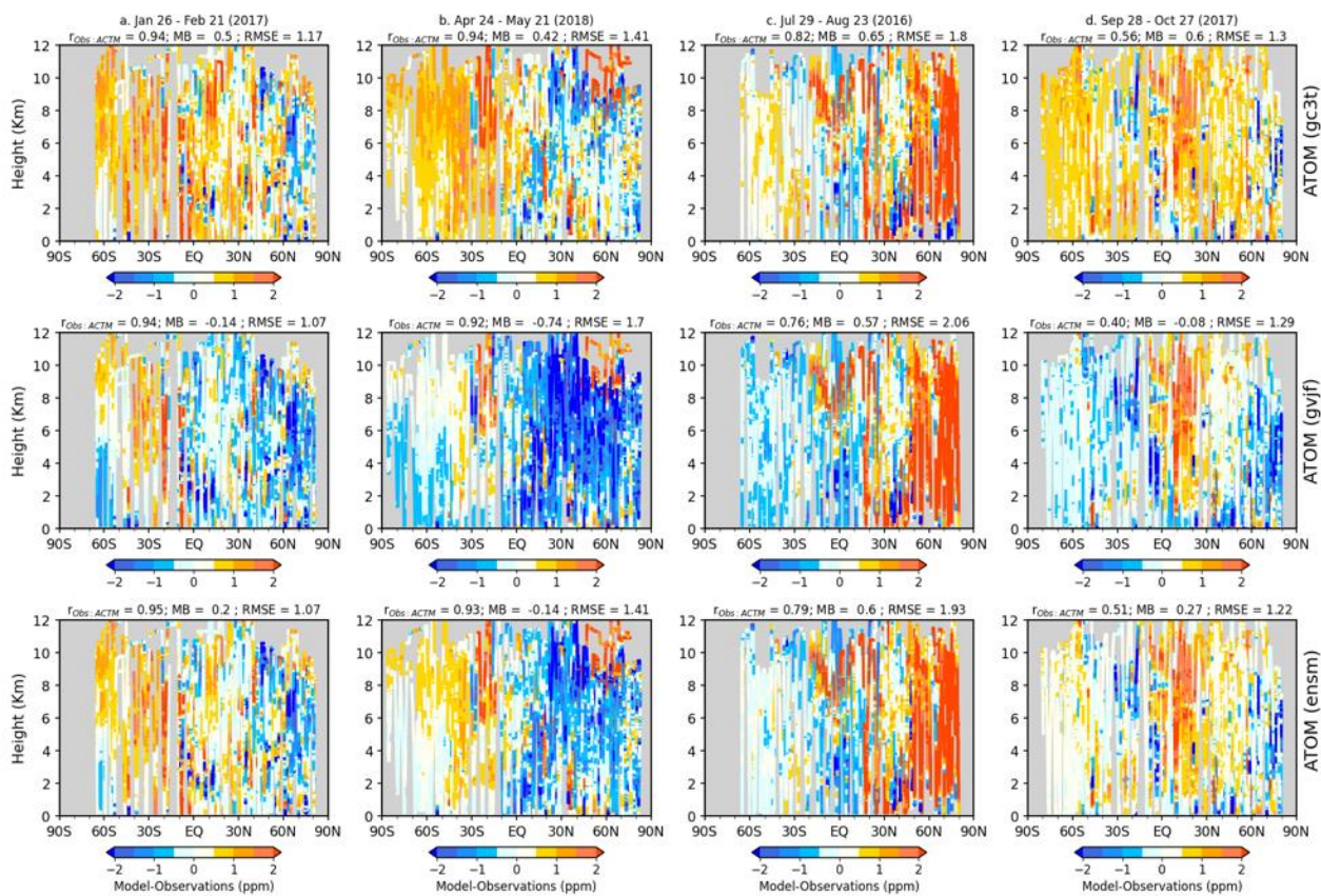
Figure S6: Same as S2, but for ATom aircraft campaigns.
