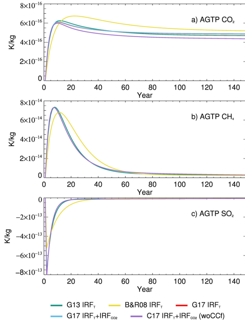
Figure S1: AGTP( t ) for CO_2 , CH_4 and SO_2 as calculated using different combinations of climate response and carbon dioxide impulse response functions: B&R08 (Boucher & Reddy, 2008), G13 (Geoffroy et al., 2013) and G17 (Gasser et al., 2017) (all with the Joos et al. (2013) CO_2 IRF), and G17 with corresponding CO_2 IRFs with and without the carbon-climate feedback included.
