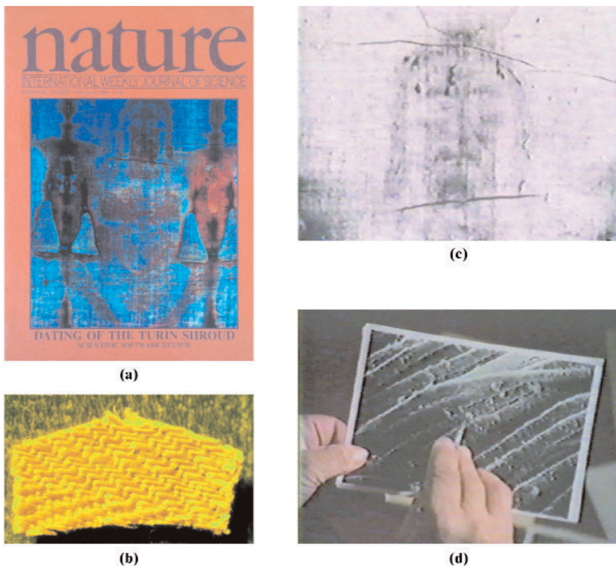
Fig. 15. The Turin Shroud. Shown in the montage are: (15a, upper left), the cover of the issue of Nature (16 February 1989) reporting the results of the ^{14}\text{C} measurements by AMS laboratories in Tucson, Zürich, and Oxford; and three singular features of the artifact: (15b, lower left), the \approx 50 mg dating sample received by the Tucson laboratory, showing the distinctive weave (3:1 herringbone twill), with dimensions about 1\text{ cm} \times 0.5\text{ cm} ; (15c, upper right), the characteristic negative image, considered by some as a remarkable piece of mediaeval art; and (15d, lower right), a microphotograph by Max Frei showing individual fibers supporting pollen grains of presumed unique origin [38, 39].
