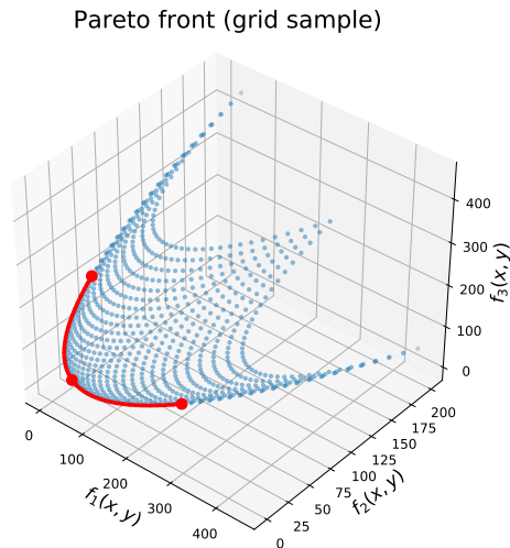
■ Figure 15 Objective space of the triobjective optimization problem presented in Figure 14: The Pareto front is outlined with a red curve. The blue points represent the image of the objective functions when the domain is sampled on a regular grid.
