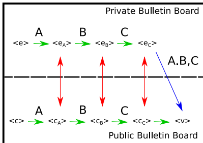
Figure: Mixing with three authorities
