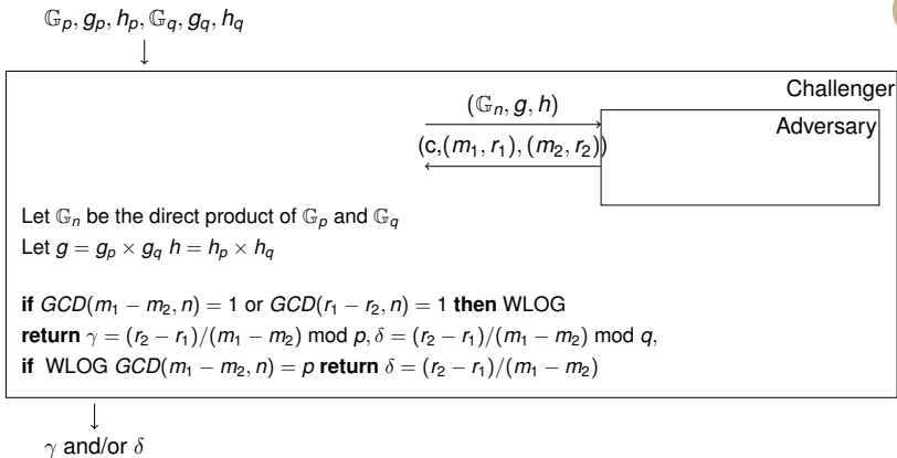
Figure: Reduction from binding to discrete log
