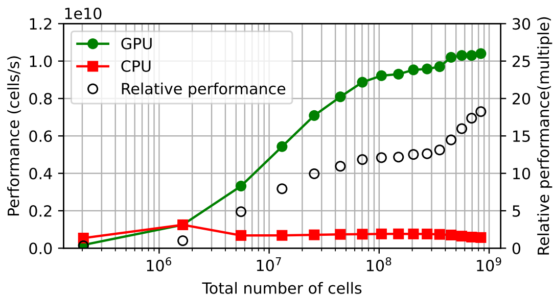
Figure 3. MPDATA single node performance comparison.
