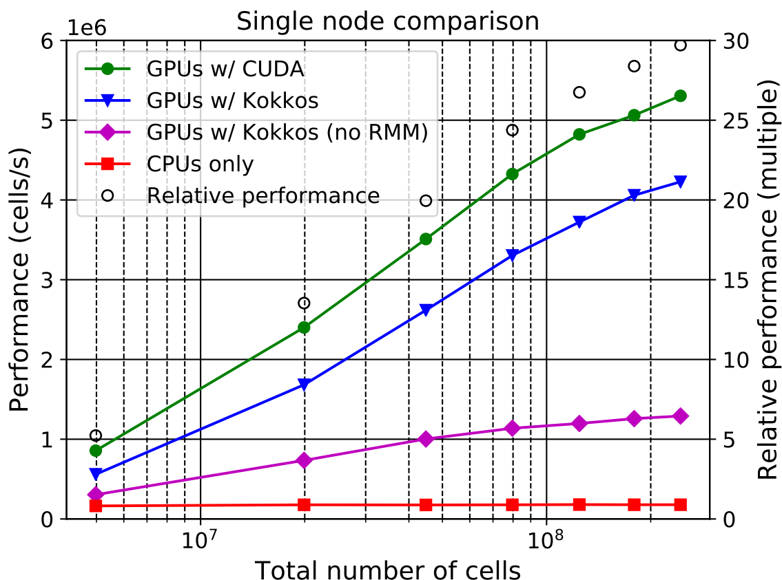
Figure 1. Parflow single node performance comparison. Relative performance refers to the performance ratio between CUDA and CPU implementations of the code. RMM denotes Rapid Memory Manager.
