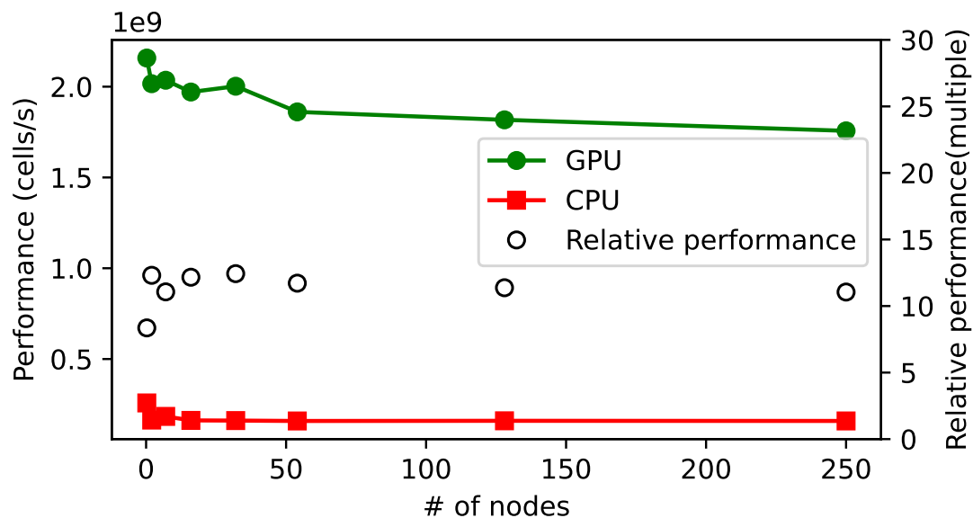
Figure 5. Weak scalability of MPDATA gauge implementation for the 492^3 -gridpoints-per-node problem size.
