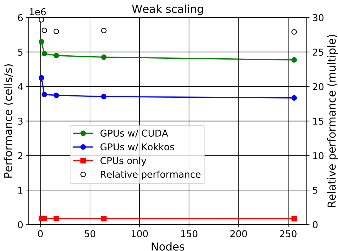
Figure 2. Weak scaling comparison.
