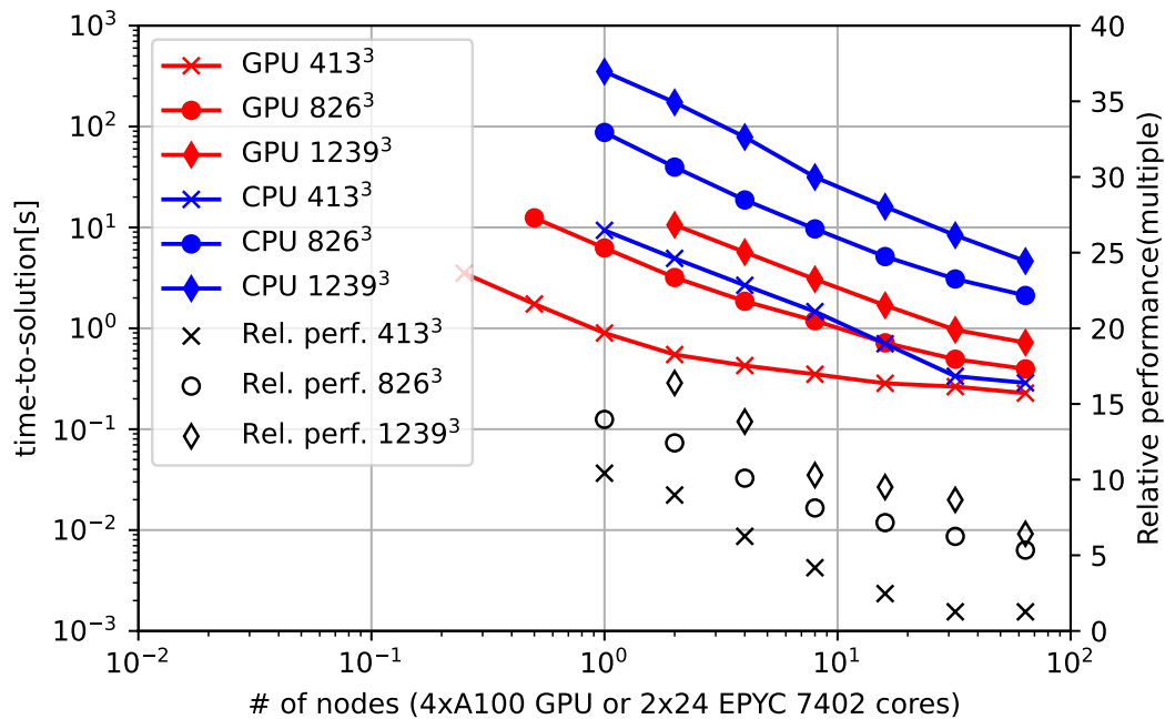
Figure 4. Strong scalability of MPDATA gauge implementation for different problem sizes. For time-to-solution (colored lines) the leftmost datapoints correspond to 1/2 and 1/4 of a 4 GPU node, i.e. 2 or 1 NVIDIA A100 GPU, respectively. Relative performance gain (point symbols) is shown for full node GPU vs. CPU simulations. Numbers in the legend denote total cell counts for the refined reference domain: (7 * 59)^3 , (14 * 59)^3 and (21 * 59)^3 .
