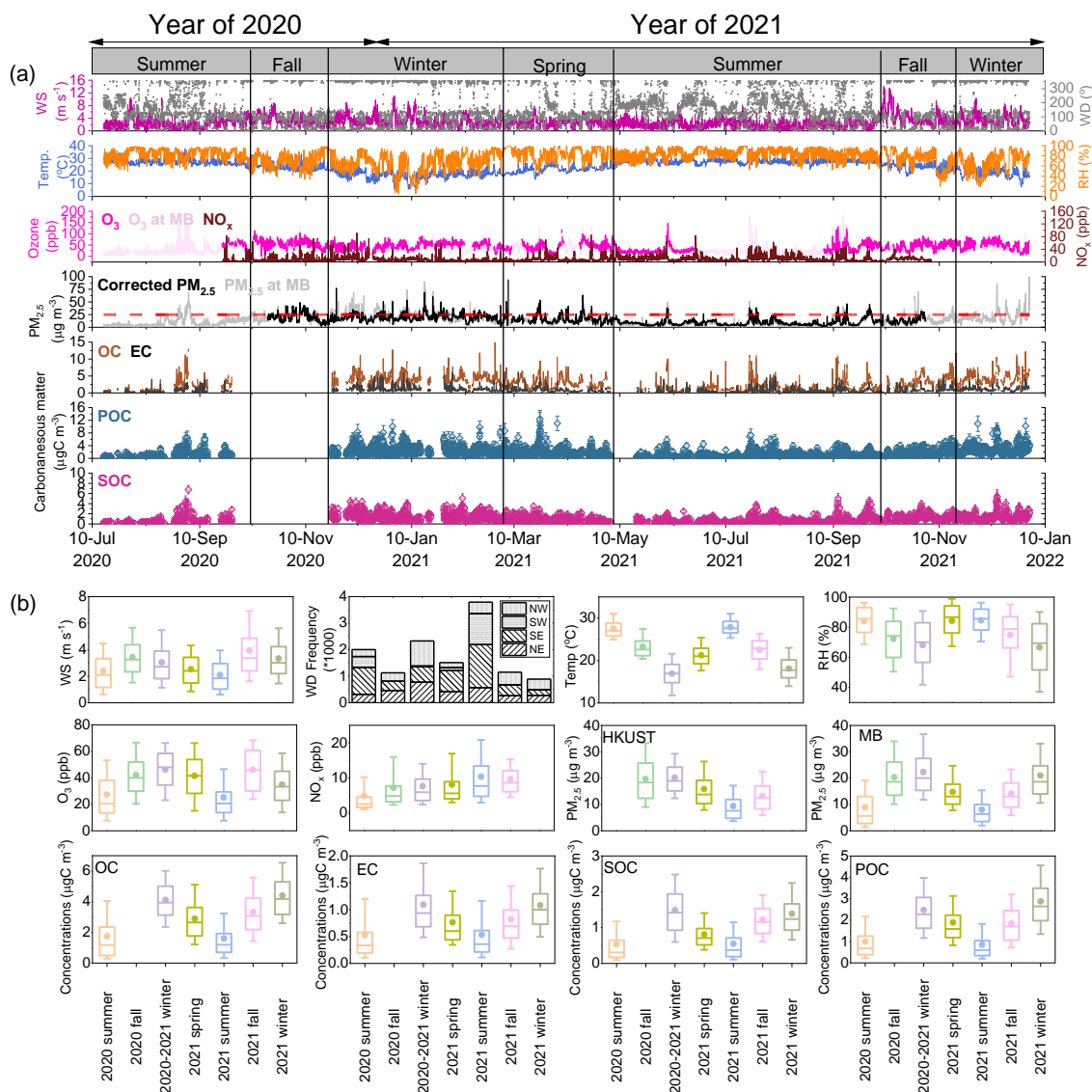
300 Figure 2. (a) Time series of meteorological parameters (wind speed, wind direction, temperature, and RH), gaseous pollutants (O 3 , and NO x ), PM 2.5 (the red dash line marks the WHO AQG IT-4 value), OC and EC, as well as POC and SOC (the y-axis error bars represent uncertainties derived from BI method) and (b) Seasonal variations (the circles and horizontal lines in the box denote the average and median, the lower and upper boundaries of the boxes represent the 25 th and 75 th percentile values, and whisker are 10 th and 90 th percentile) during the observation period (16 July 2020–31 December 2021) at the HKUST supersite.
