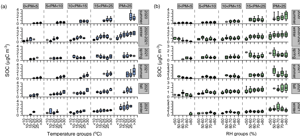
Figure 4. Concentrations of SOC as a function of (a) temperature bins and (b) RH bins under different PM_{2.5} groups in individual seasons during the entire measurement period. The markers represent the mean values, and whiskers represent the 25 th and 75 th percentiles.
