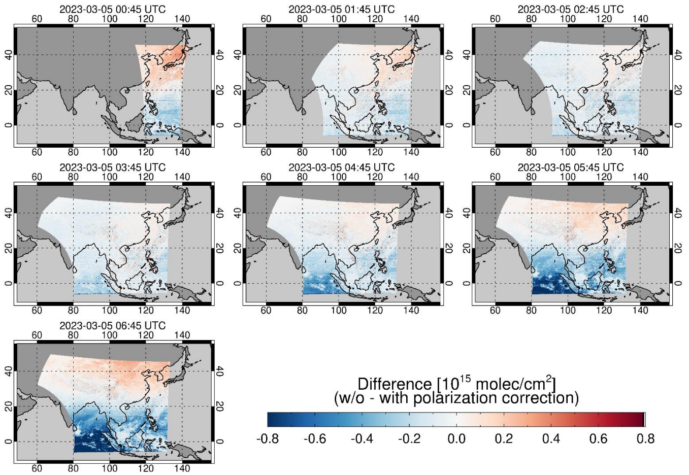
880 Figure A3: The diurnal variation of the difference in GEMS geometric NO 2 vertical columns without and with polarization correction on 5 March 2023 from 00:45 to 06:45 UTC.
