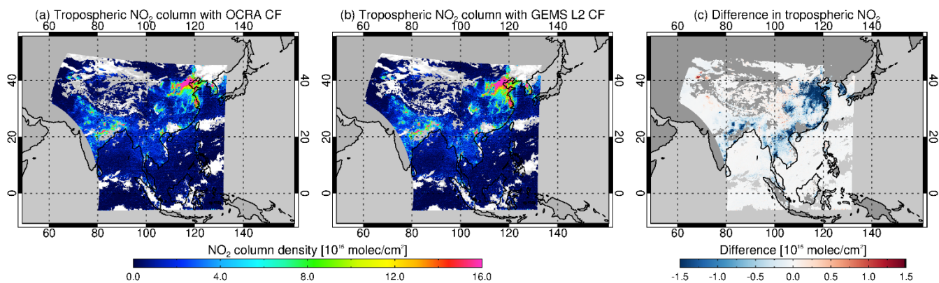
420 Figure 9: Tropospheric NO 2 columns retrieved using (a) OCRA cloud fractions (displayed in Fig. 8a), and (b) GEMS L2 v2.0 cloud fractions (displayed in Fig. 8b) for 14 March 2023 at 04:45 UTC. (c) Differences in tropospheric NO 2 columns applying the OCRA-based cloud corrections and GEMS L2 O 2 -O 2 based cloud corrections (a – b in this figure). Only measurements with cloud fraction \leq 0.4 are included.
