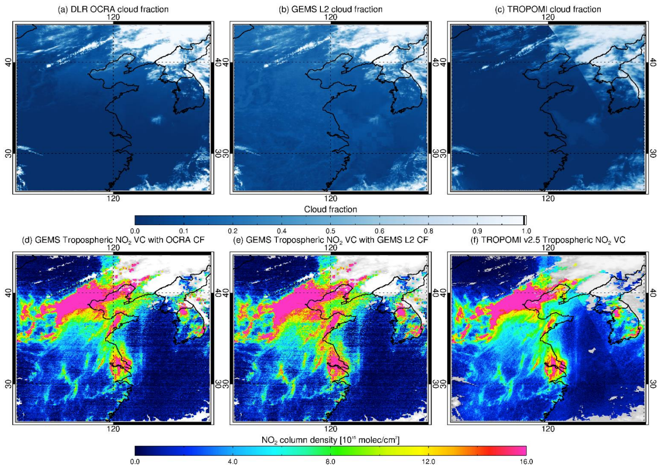
425 Figure 10: Zoomed maps for cloud fractions from (a) OCRA adapted to GEMS level 1 data, (b) GEMS L2 v2.0 cloud product, and (c) TROPOMI L2 v2.4 cloud product over polluted areas including eastern China and Korea peninsula for 14 March 2023 at 04:45 UTC. GEMS tropospheric NO 2 vertical columns retrieved using (d) OCRA cloud fractions (displayed in Fig. 10a) and (e) GEMS L2 v2.0 cloud fractions (displayed in Fig. 10b). (f) TROPOMI L2 v2.5 tropospheric NO 2 columns for the corresponding scene.
