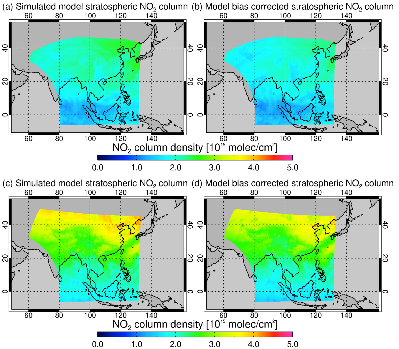
310 Figure 6: Simulated model stratospheric NO 2 vertical columns by CAMS forecast (a, c) and the bias-corrected modelled stratospheric NO 2 vertical columns (b, d) on 10 December 2022 (a, b) and 10 June 2023 (c, d).
