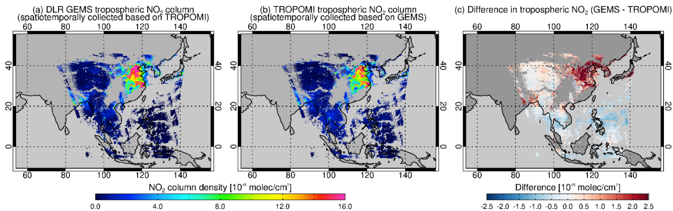
645 Figure 19: Same as Fig. 18, but for 14 December 2022.
