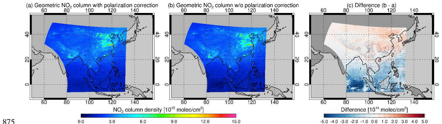
Figure A2: GEMS geometric NO 2 vertical columns retrieved (a) with and (b) without polarization correction, and (c) the differences between the two (b - a) for 15 March 2023 at 04:45 UTC.
