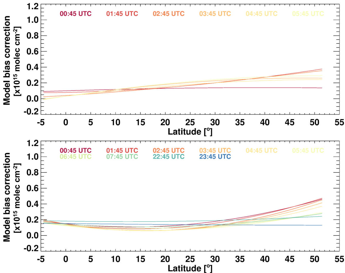
Figure 5: Model bias correction terms parameterized as a function of latitude for each scan time on 10 December 2022 (top) and 10 June 2023 (bottom), respectively.
