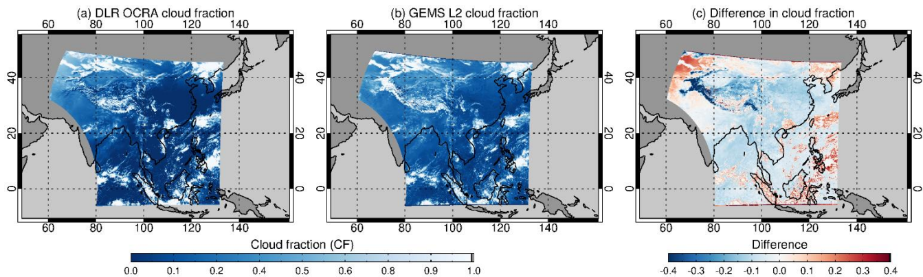
415 Figure 8: Maps of cloud fractions from (a) OCRA adapted to GEMS level 1 data, and (b) GEMS L2 v2.0 cloud product for 14 March 2023 at 04:45 UTC. (c) Differences in cloud fractions (OCRA – GEMS L2 v2.0; a – b in this figure) for the corresponding scene.
