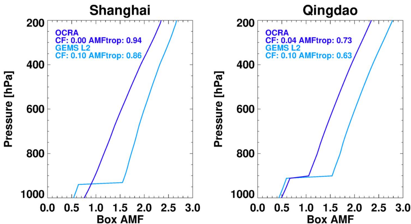
430 Figure 11: Comparisons of box-AMFs derived using the OCRA and GEMS L2 v2.0 cloud fraction for clear-sky scenes over Shanghai (32.22 °N, 121.37 °E) and Qingdao (35.05 °N, 119.57 °E) in eastern China on 14 March 2023 at 04:45 UTC. Cloud fractions and calculated tropospheric AMFs for each case are denoted.
