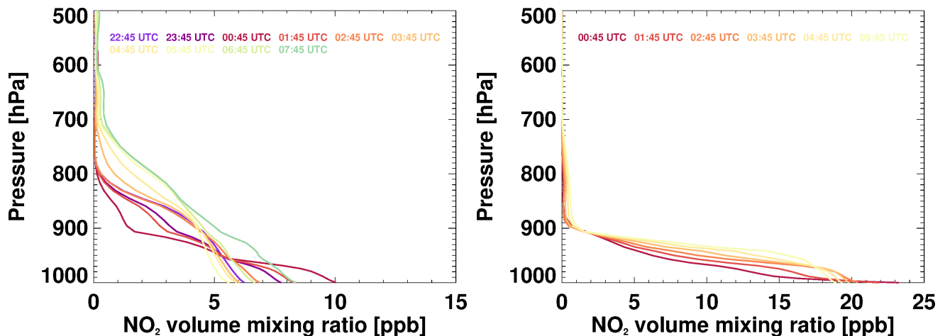
Figure 16: A priori NO 2 profiles from the CAMS forecast model for GEMS each scan hour over the Seoul metropolitan area (37.53° N, 120.01 °E) on 15 June 2023 (left) and 12 December 2022 (right), respectively.
