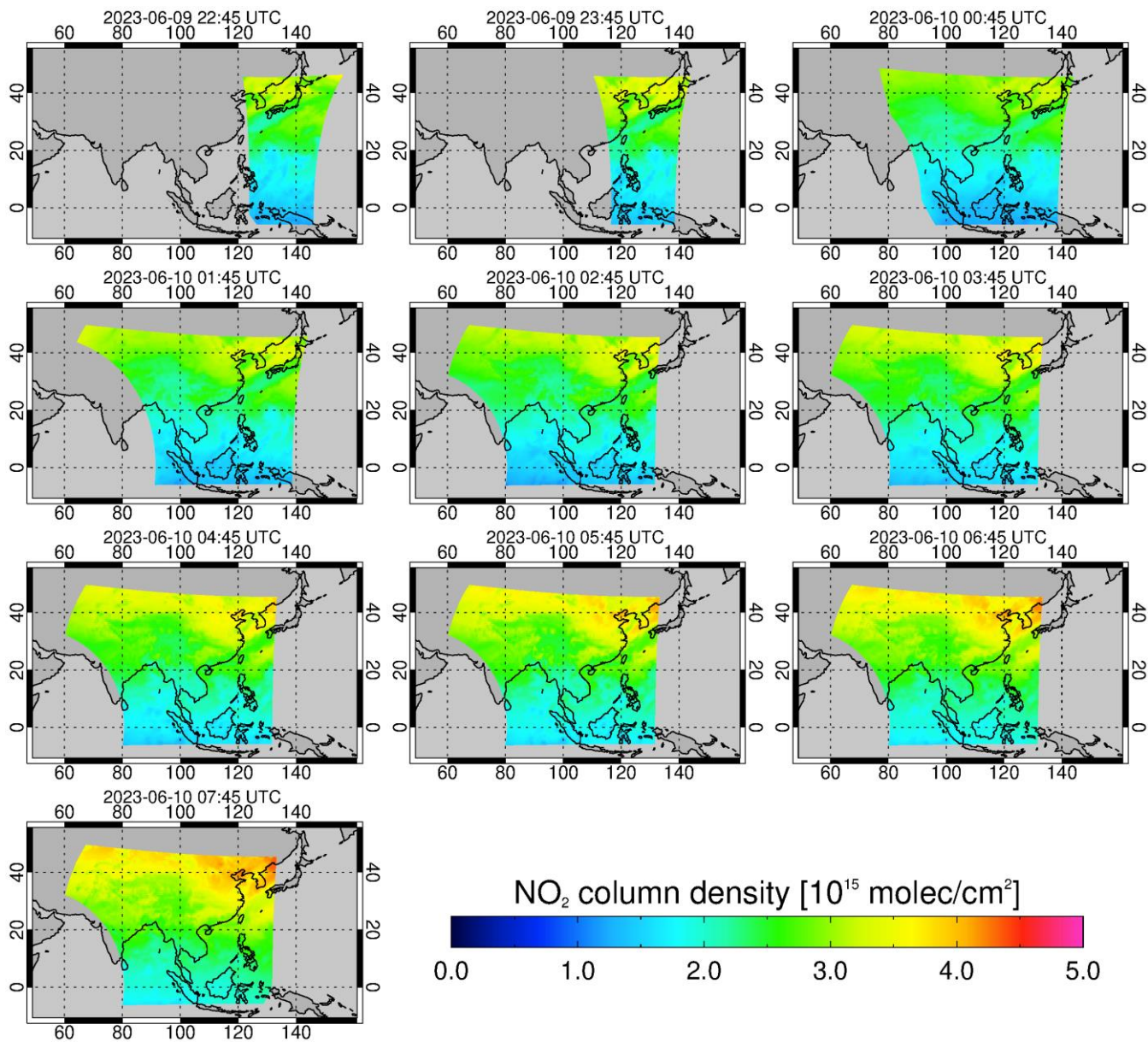
315 Figure 7: Diurnal variation of estimated stratospheric NO 2 columns based on the approach utilizing the CAMS forecast model profile data (described in Sect. 2.2.2) on 10 June 2023.
