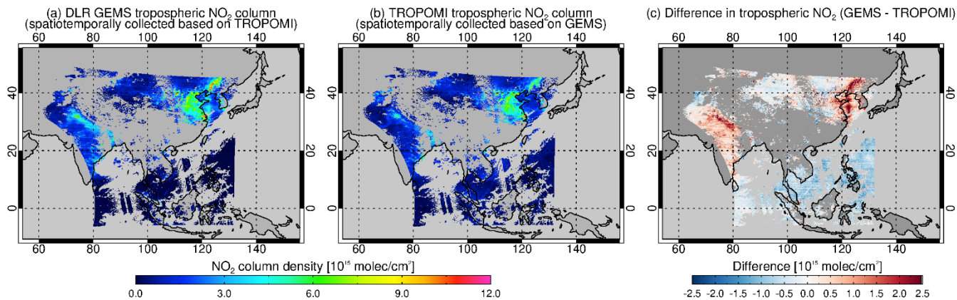
640 Figure 18: Comparison between DLR GEMS and TROPOMI operational v2.4 tropospheric NO 2 columns on 14 June 2023. Only measurements with cloud radiance fractions < 0.5 are included. Both tropospheric NO 2 columns are regridded to a 0.1° × 0.1° resolution based on temporally and spatially collocated data for the corresponding date.
