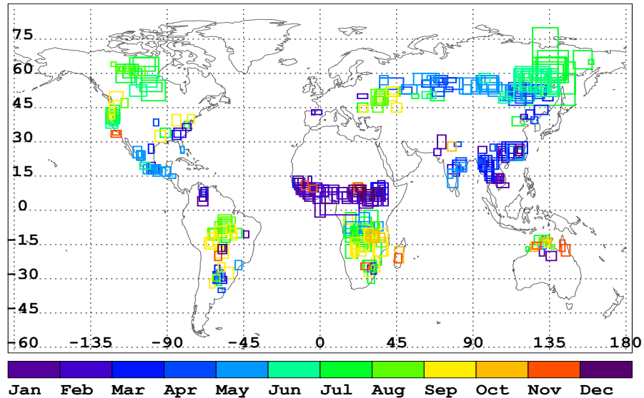
Figure 2: Locations and months of the fire case boxes in this study.
