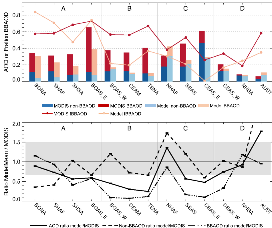
385 Figure 6: Top: Total AOD from MODIS (stacked dark red and blue-shaded bars) and from multi-model mean (light stacked red and blue-shaded bars), the corresponding BBAOD (red colors) and non-BB background AOD (blue colors), and their BB AOD fractions (lines), averaged for cases in each of the 13 regions grouped by A, B, C, and D (see Fig. 5 and text). Bottom: Ratios of model mean to MODIS for total AOD (solid line), BB AOD (dot-dashed line, and non-BB background AOD (dashed line). The light gray shade indicates the range of model to MODIS ratio (R) within 50% ( 0.67 \leq R \leq 1.5 ).
