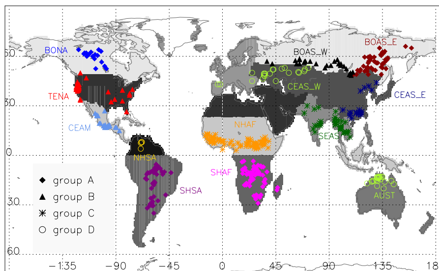
Figure 3: The 13 regions with the BB cases in each region. BONA = Boreal North America, TENA = Temperate North America, CEAM = Central America, NHSA = Northern Hemisphere South America, SHSA = Southern Hemisphere South America, NHAF = Northern Hemisphere Africa, SHAF = Southern Hemisphere Africa, BOAS_W = Boreal Asia West, BOAS_E = Boreal Asia East, CEAS_W = Central Asia West, CEAS_E = Central Asia East, SEAS = Southeast Asia, AUST = Australia. Symbols for BB cases mark the group (A, B, C or D) that the BB region belongs to. The groups of BB regions are explained in section 3.2.
