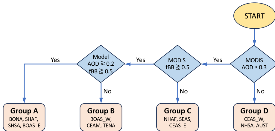
Figure 5: Flow chart of the procedure used to separate the 13 biomass burning regions into four groups having distinct characteristics in biomass burning intensity, fraction of smoke AOD w.r.t. total AOD (fBB), and differences between the quantities from MODIS and the multi-model mean. Regions in each group and their characteristics are shown in Fig. 6.
