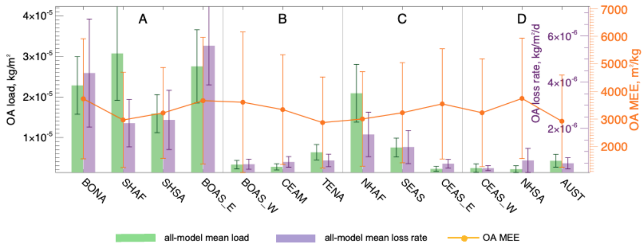
Figure 7: Multi-model mean BB OA load (kg/m²; green bars, left Y axis), multi-model mean BB OA loss rate (kg/m²-day; purple bars, right purple Y axis), and multi-model mean mass extinction efficiency of BB OA (m²/kg; orange points and whiskers, right orange Y axis) averaged for cases in each of the 13 regions grouped by A, B, C, and D (see Fig. 5 and text). Whiskers show standard deviations of the multi-model means, respectively.
